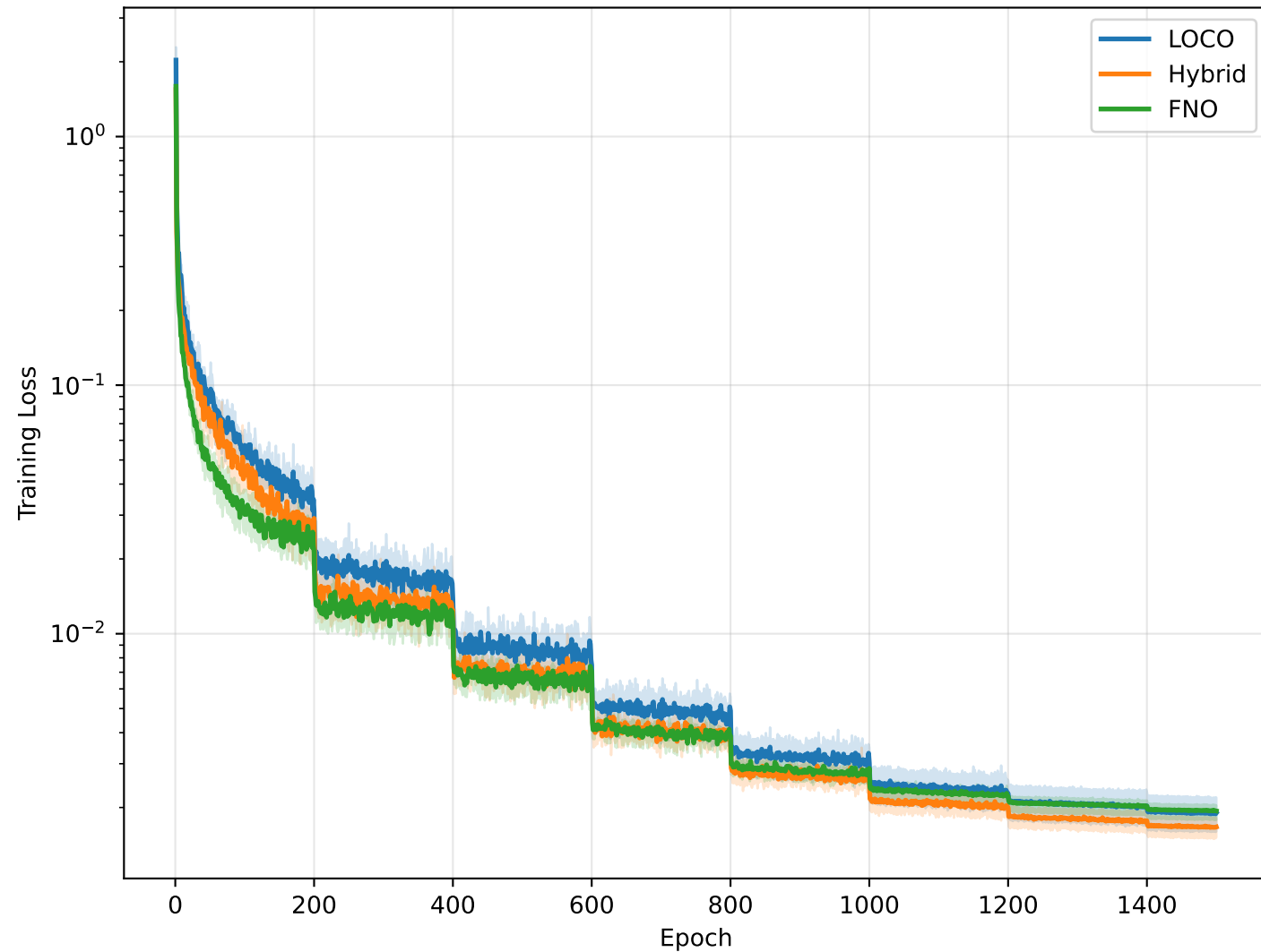
Training Loss (Mean + 10th-90th Percentile)
