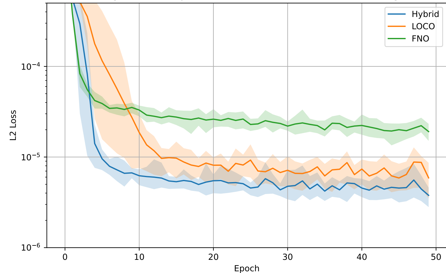
Training Loss Over Epochs (Mean + 10th-90th Percentile) - Burgers
