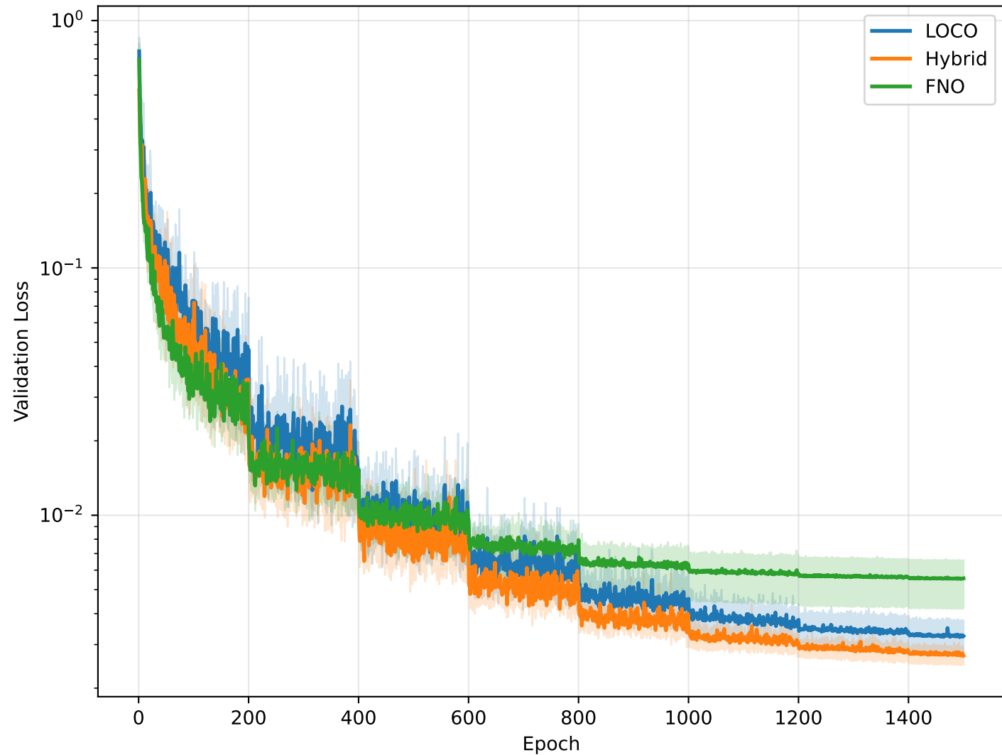
Validation Loss (Mean + 10th-90th Percentile)
