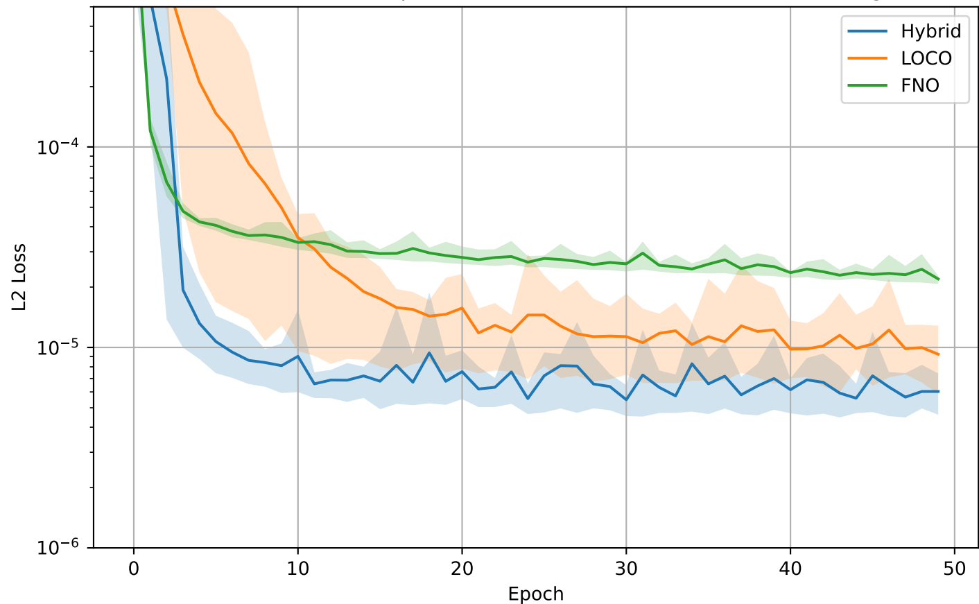
Validation Loss Over Epochs (Mean + 10th-90th Percentile) - Burgers
