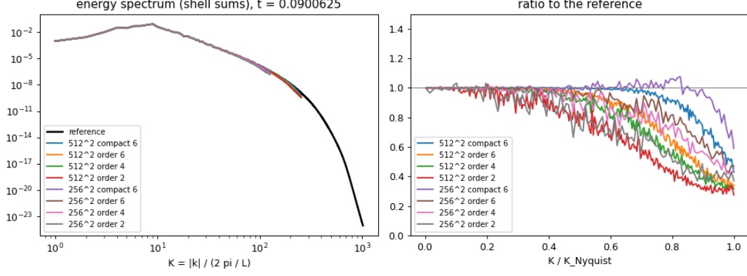
Figure 6: Decaying turbulence at t = 0.09 : energy spectra of 256^2 and 512^2 runs with orders 2, 4 and 6 and the compact scheme, and their ratio to a 2048^2 order-6 run.
