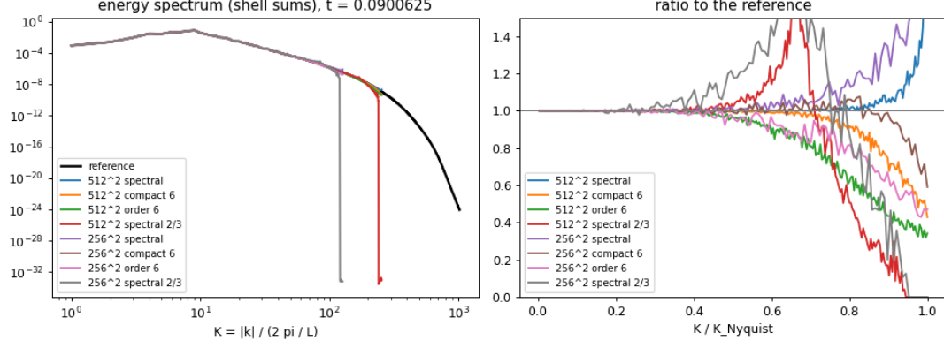
Figure 4: As fig. 6, with pseudospectral differentiation, with and without the 2/3 rule.
