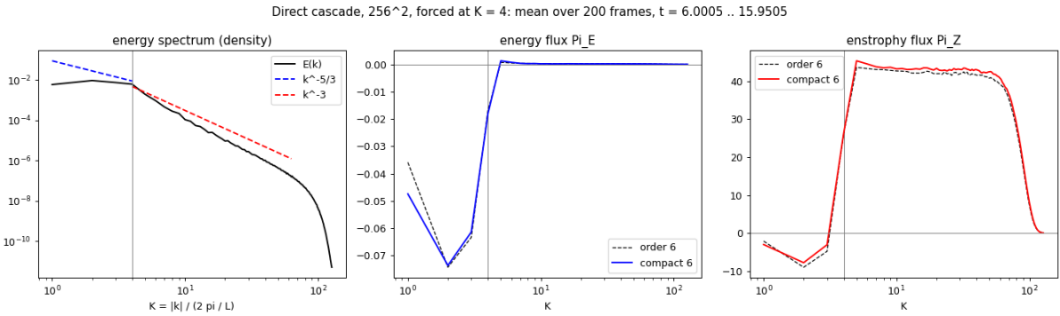
Figure 5: Direct cascade on 256^2 with the compact scheme: time-mean spectrum and fluxes; dashed, explicit order 6.
