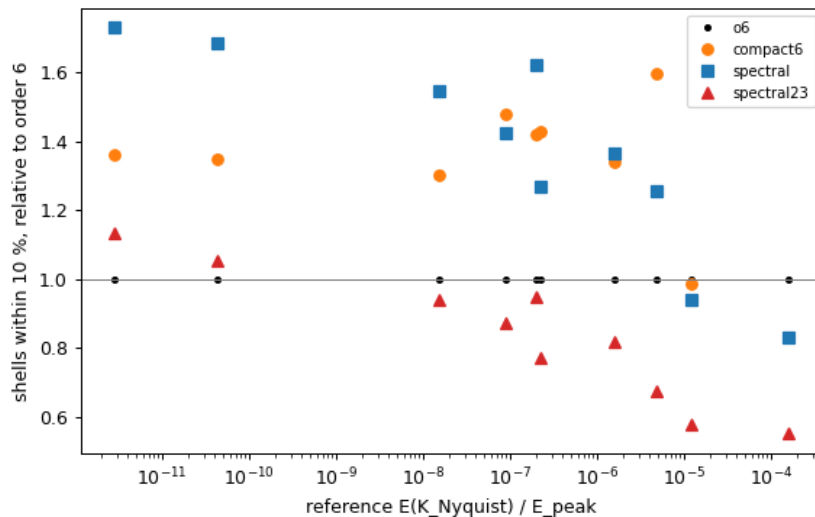
Figure 5: Shells within 10% of the reference, relative to explicit order 6, against the reference’s energy at the grid’s Nyquist shell relative to its peak: five decaying cases ( \text{Re} and k_0 varied about the baseline) on 256^2 and 512^2 .
