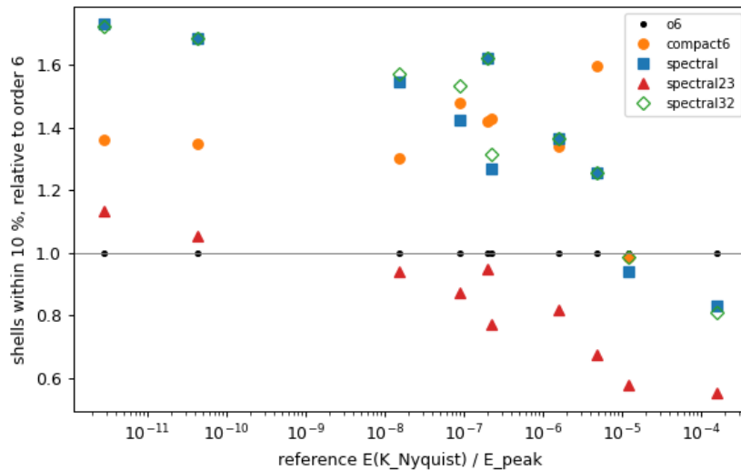
Figure 5: Shells within 10 % of the reference, relative to explicit order 6, against the reference’s energy at the grid’s Nyquist shell relative to its peak: five decaying cases ( \text{Re} and k_0 varied about the baseline) on 256^2 and 512^2 . Open diamonds: pseudospectral with 3/2 padding, on top of the undealiased squares.
