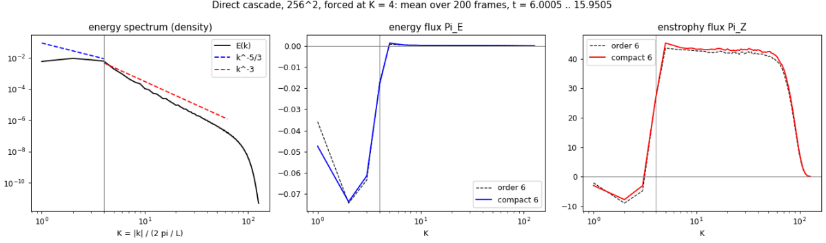
Figure 4: Direct cascade on 256^2 with the compact scheme: time-mean spectrum and fluxes; dashed, explicit order 6.
