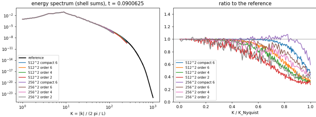
Figure 5: Decaying turbulence at t = 0.09 : energy spectra of 256^2 and 512^2 runs with orders 2, 4 and 6 and the compact scheme, and their ratio to a 2048^2 order-6 run.
