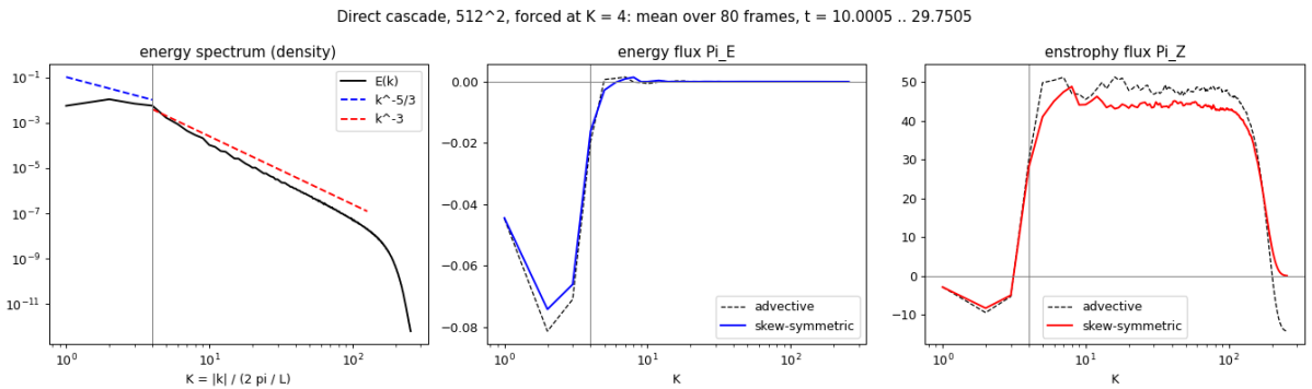
Figure 1: Direct cascade: time-mean energy spectrum (with k^{-5/3} and k^{-3} for reference) and fluxes, skew-symmetric form; dashed, the advective form.
