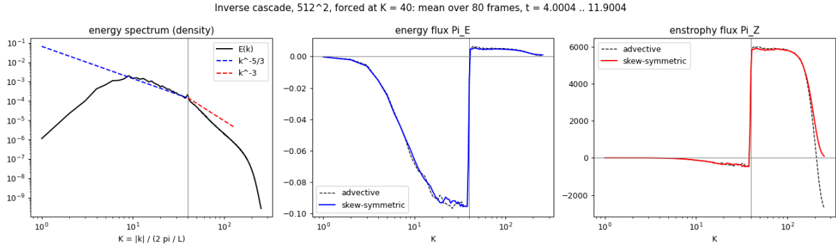
Figure 2: Inverse cascade: as fig. 1, forced at K = 40 .
