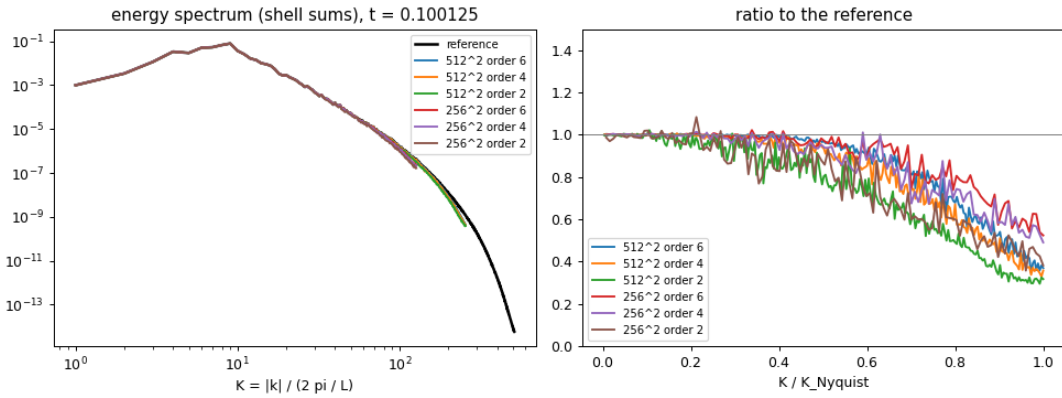
Figure 4: Decaying turbulence at t = 0.1 : energy spectra of 256^2 and 512^2 runs with orders 2, 4 and 6, and their ratio to a 1024^2 order-6 run.
