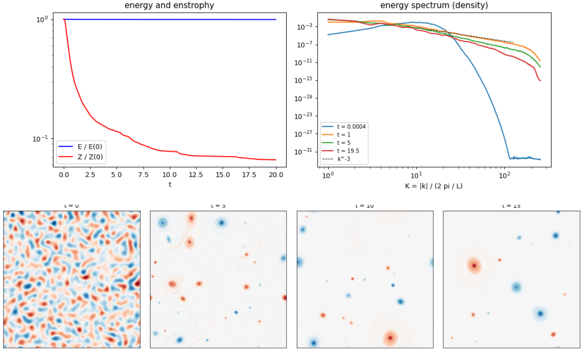
Figure 3: Decaying turbulence on 512^2 : energy and enstrophy, energy spectra, and the vorticity at t = 0, 5, 10 and 15 .
