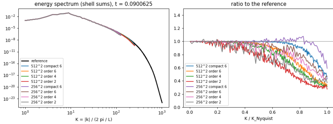
Figure 7: Decaying turbulence at t = 0.09 : energy spectra of 256^2 and 512^2 runs with orders 2, 4 and 6 and the compact scheme, and their ratio to a 2048^2 order-6 run.
