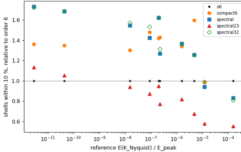
Figure 5: Shells within 10 % of the reference, relative to explicit order 6, against the reference’s energy at the grid’s Nyquist shell relative to its peak: five decaying cases (Re and k_0 varied about the baseline) on 256^2 and 512^2 . Open diamonds: pseudospectral with 3/2 padding, on top of the undealiased squares.
