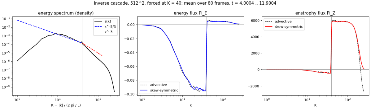
Figure 2: Inverse cascade: as fig. 1, forced at K = 40 .
