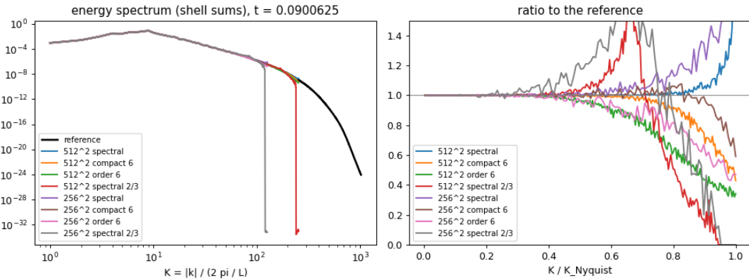
Figure 4: As fig. 7, with pseudospectral differentiation, with and without the 2/3 rule.
