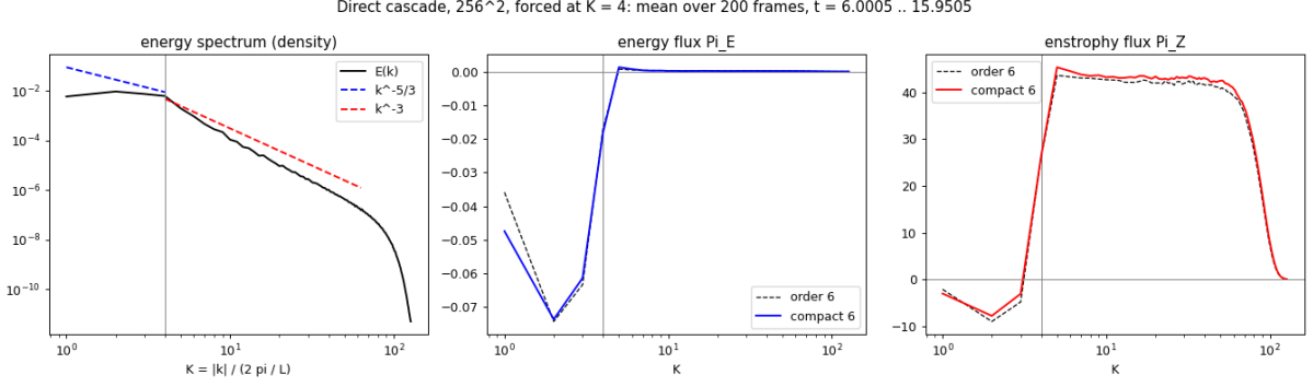
Figure 6: Direct cascade on 256^2 with the compact scheme: time-mean spectrum and fluxes; dashed, explicit order 6.
