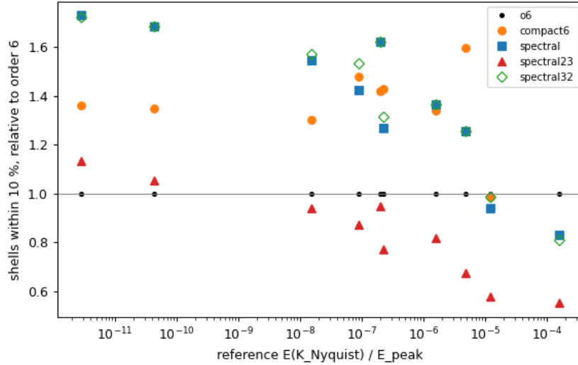
Figure 5: Shells within 10 % of the reference, relative to explicit order 6, against the reference’s energy at the grid’s Nyquist shell relative to its peak: five decaying cases ( Re and k_0 varied about the baseline) on 256^2 and 512^2 . Open diamonds: pseudospectral with 3/2 padding, on top of the undealiased squares.
