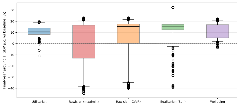
Figure 4: Distribution over the 110 provinces of final-year GDP per capita change versus the baseline scenario, per ethical framework (boxes: quartiles; whiskers: 5th–95th percentile). The frameworks differ not only in their means but in the shape of who benefits.
