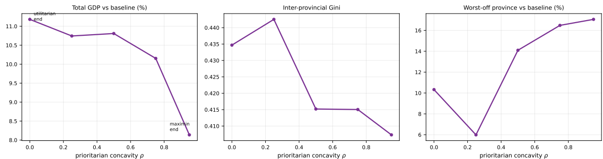
Figure 7: Prioritarian sweep: final-year total GDP (left), inter-provincial Gini (center), and the worst-off province (right) as the concavity \rho rises from the utilitarian end ( \rho=0 ) toward maximin. Means over 3 seeds. The single parameter traces the efficiency–equity continuum as a curve.
