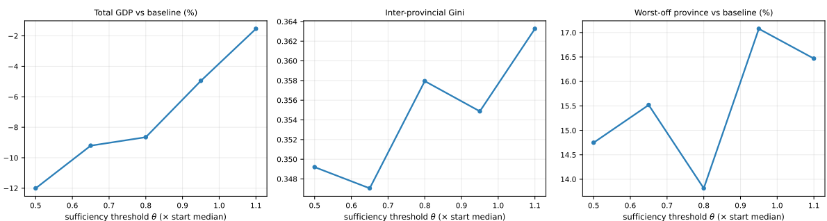
Figure 8: Sufficiency sweep: final-year total GDP (left), Gini (center), and the worst-off province (right) as the sufficiency threshold \theta rises. Means over 3 seeds. Raising the “enough” line shifts the optimizer’s effort toward the floor.
