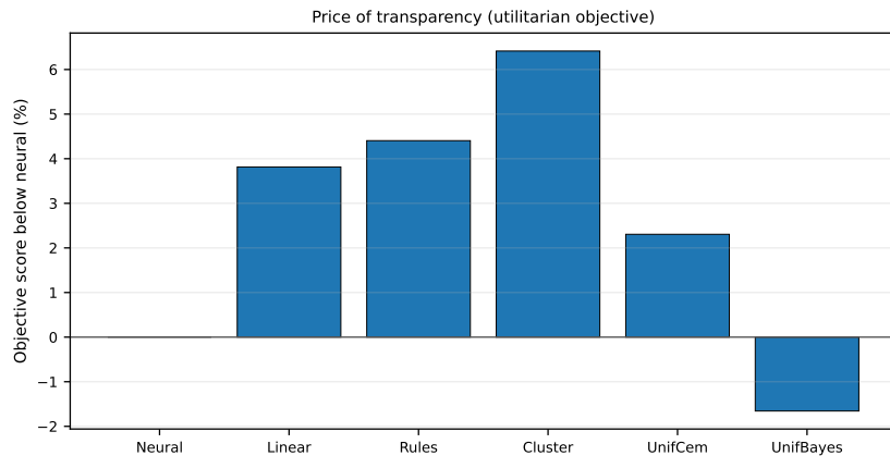
Figure 9: The score gap to the neural policy for each model (utilitarian objective, 3 seeds). Shorter bars are cheaper transparency; the white-box models give up little.
