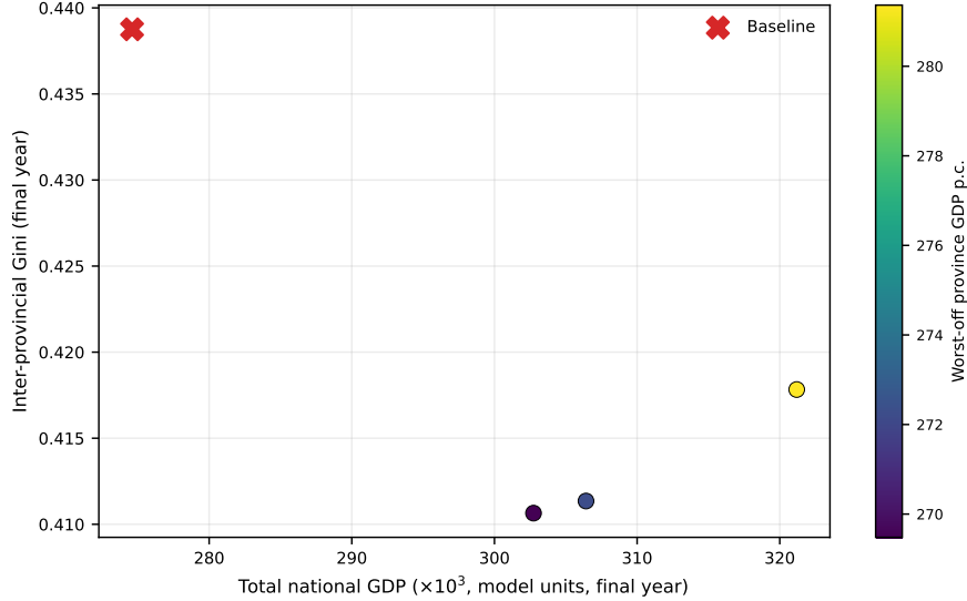
Figure 6: NSGA-II over per-cluster lever vectors (4 k-means regional packages; 6 generations, population 12). Unlike the uniform front, this one spans a real range of inequality (Gini 0.411–0.418), so efficiency (horizontal) and equity (vertical) are genuinely in tension; colour encodes the worst-off province’s GDP. The red cross marks the baseline. Targeting — not the overall intensity of national policy — is what opens the trade-off.
