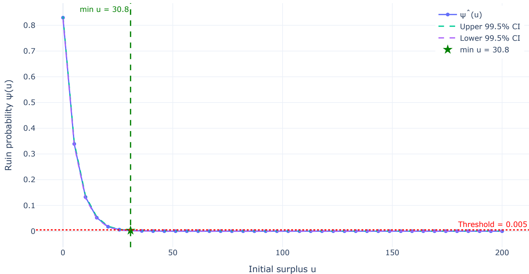
Minimum Surplus for \psi(u) < 0.005 (99.5% CI)
