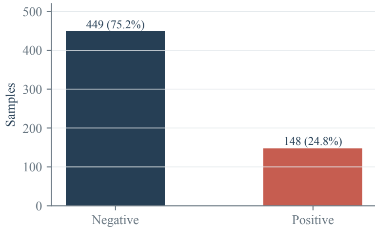
Class balance
