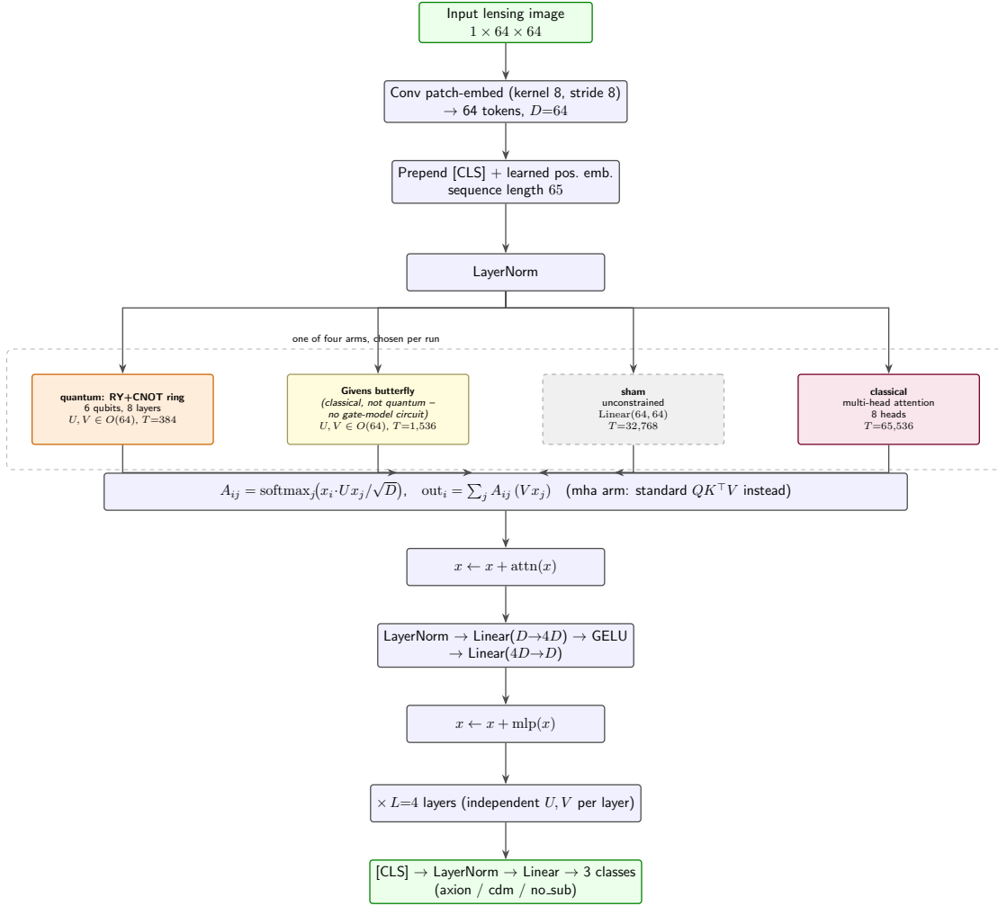
Figure 1: QOVT pipeline. All four attention arms (RY+CNOT: quantum; Givens butterfly, sham, classical MHA: all classical) share an identical backbone and differ only in how U, V (or, for the classical arm, Q, K, V ) are computed inside each of the L=4 attention layers – one arm is trained per run.
