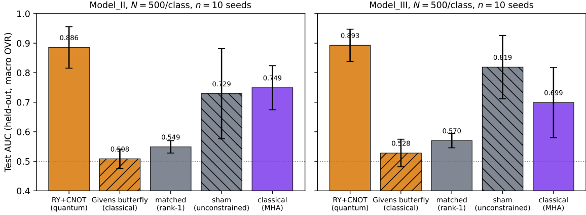
Figure 2: Pre-registered ablation results (Table 8), mean \pm std over 10 seeds. RY+CNOT is the only arm that trains reliably above chance at N=500 under this protocol; Givens butterfly does not.
