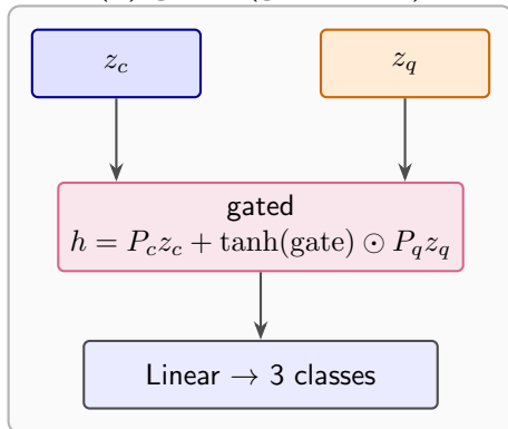
(b) gated (gate init 0)
