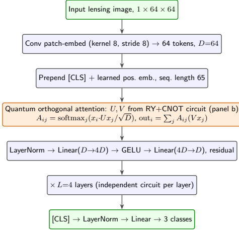
Figure 1: The quantum arm of QOVT. (a) End-to-end pipeline: only the quantum RY+CNOT circuit is shown as the source of U, V – classical controls (Givens butterfly, sham, classical MHA) are described separately in Section 2.5 and are not part of this architecture diagram. (b) The RY+CNOT ring circuit itself, one of the L_{\text{circ}}=8 repeated layers: an RY rotation on every qubit followed by a ring of nearest-neighbor CNOTs (including the wrap-around q_5 \rightarrow q_0 gate).
