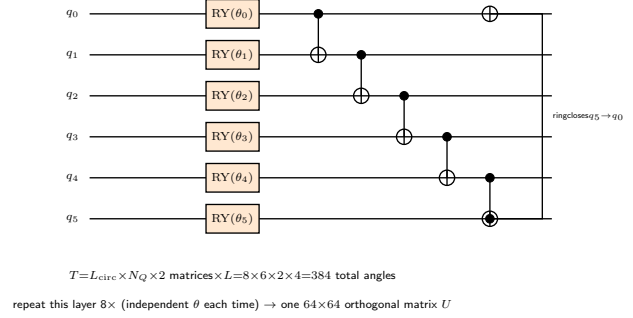
(b) RY+CNOT ring circuit (one of L_{\text{circ}}=8 layers)
