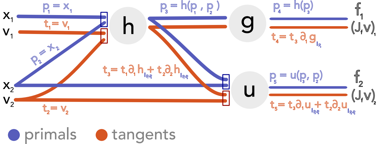
Figure 24: Illustrated is the forward differentiation through the function f (given in Eq. 238). The computational graph is evaluated from left to right, the tangent expressions correspond to the terms of the Jacobian-vector product as given in Eq. 239.
