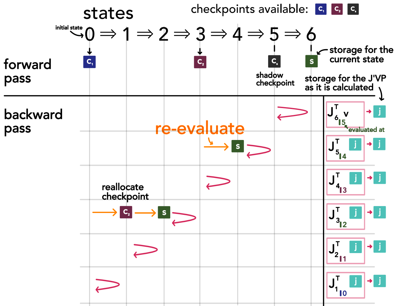
Figure 26: Illustrated is the calculation of a Jacobian transpose vector product (JVP) using checkpointing through a loop with six iterations and with two checkpoints available. The illustration is based on Fig. 2.1 in Stumm and Walther, 2010. To calculate the derivative of a state in the sequence with respect to its inputs (i.e. the previous state), these inputs must be recalculated from checkpoints. We start out with state 0 and 3 checkpointed and state 5 stored as a shadow checkpoint (we assume that in the iteration we store the current and last state). With state 5 known we can differentiate state 6. In the next step we have to reconstruct state 4 from the checkpoint at state 3 to differentiate state 5 and so forth. Checkpoints can be reallocated to reduce the number of necessary recomputations.
