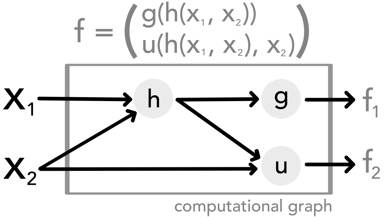
Figure 23: Illustrated is the computational graph of a function f : \mathbb{R}^2 \rightarrow \mathbb{R}^2 (given in Eq. 238) which is composed of functions g : \mathbb{R} \rightarrow \mathbb{R} , h : \mathbb{R}^2 \rightarrow \mathbb{R} , u : \mathbb{R}^2 \rightarrow \mathbb{R} depicted as nodes in the computational graph. Input relations are depicted as arrows.
