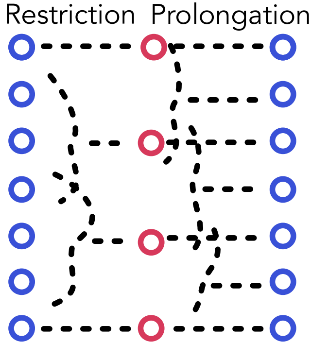
Figure 11: Illustration of restriction and prolongation.
