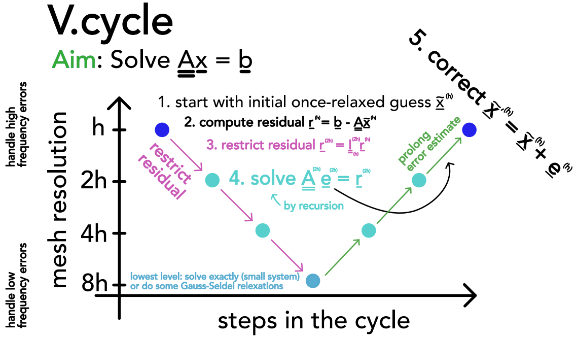
Figure 24: V-cycle.
