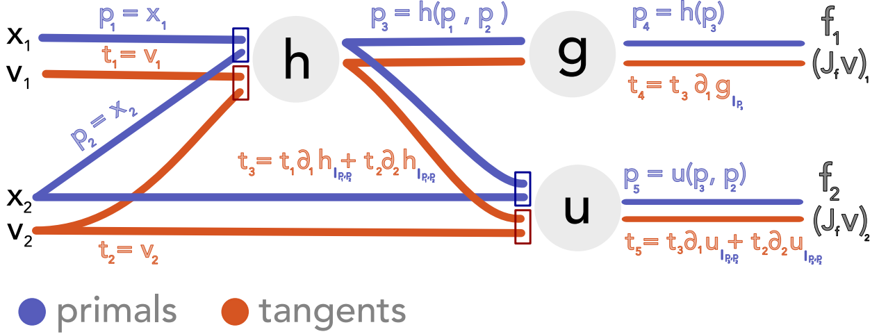
Figure 24: Illustrated is the forward differentiation through the function f (given in Eq. 224). The computational graph is evaluated from left to right, the tangent expressions correspond to the terms of the Jacobian-vector product as given in Eq. 225.
