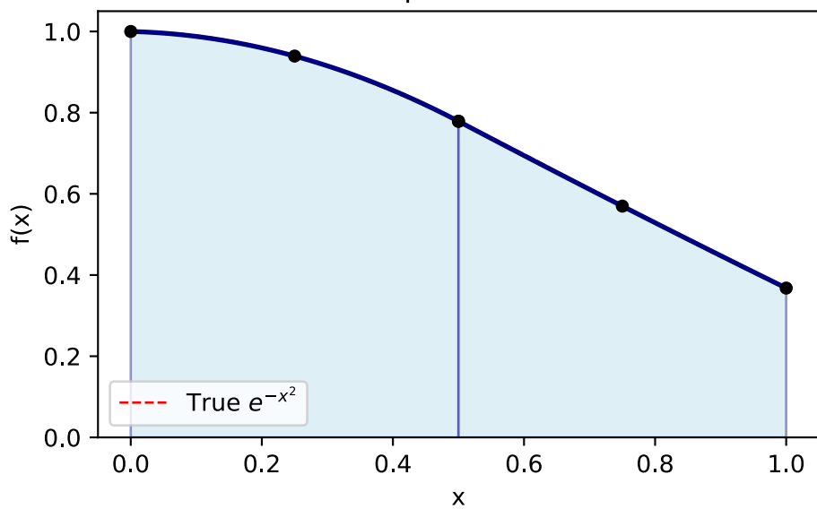
Simpson's Rule
