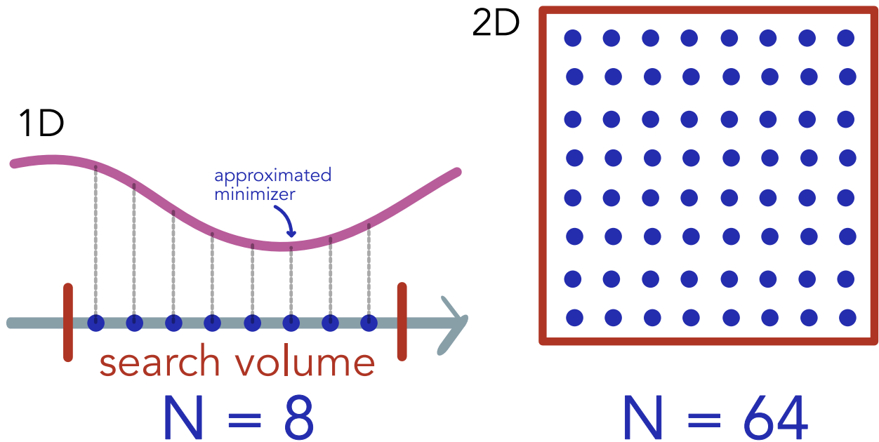
Figure 9: Curse of dimensionality in grid-search.
