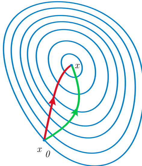
Figure 10: Newton optimization (red), gradient descent (green).
