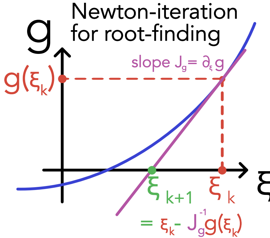
Figure 8: Illustration of the Newton-Raphson method.
