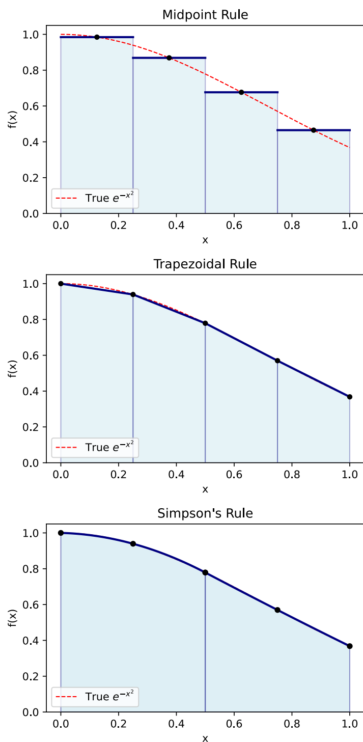
Figure 12: Comparison of the midpoint rule, trapezoidal rule and Simpson's rule for the same number of evaluation points of f .
