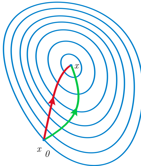
Figure 28: Newton optimization (green), gradient descent (red).
