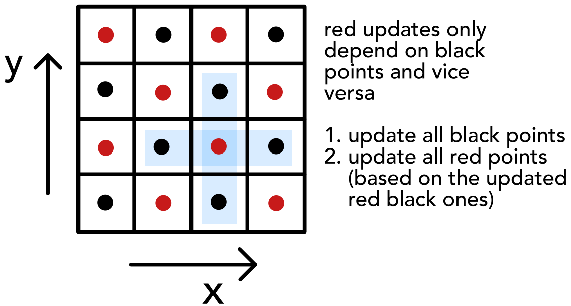
Figure 9: Red-black ordering for the 2D Poisson equation.
