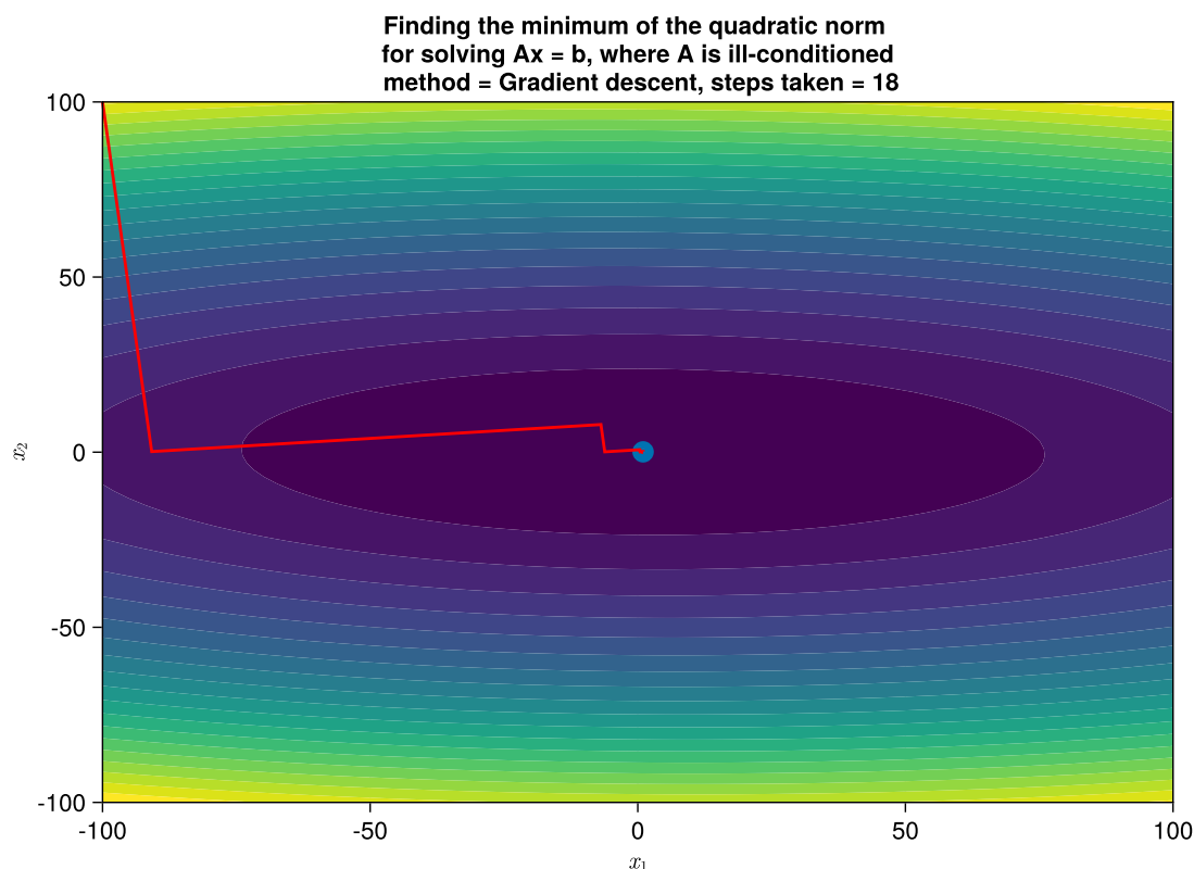
Figure 17: Steepest descent for solving a linear system \underline{\underline{A}}x = \underline{b} with positive definite matrix \underline{\underline{A}} .
