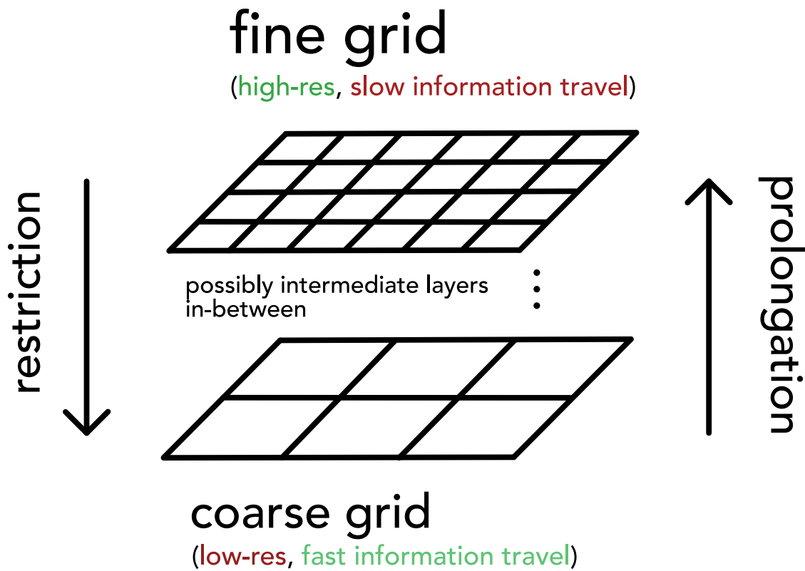
Figure 10: Grids of different resolution.
