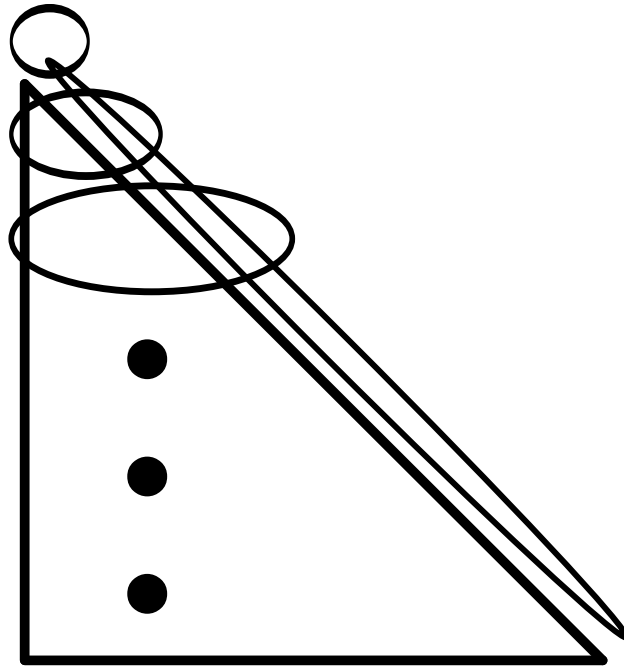
Figure 8: As of \underline{\underline{L}}\underline{\underline{x}}^{(n+1)} to calculate x_i^{(n+1)} we only need x_0^{(n+1)}, \dots, x_{i-1}^{(n+1)} which we have already calculated.
