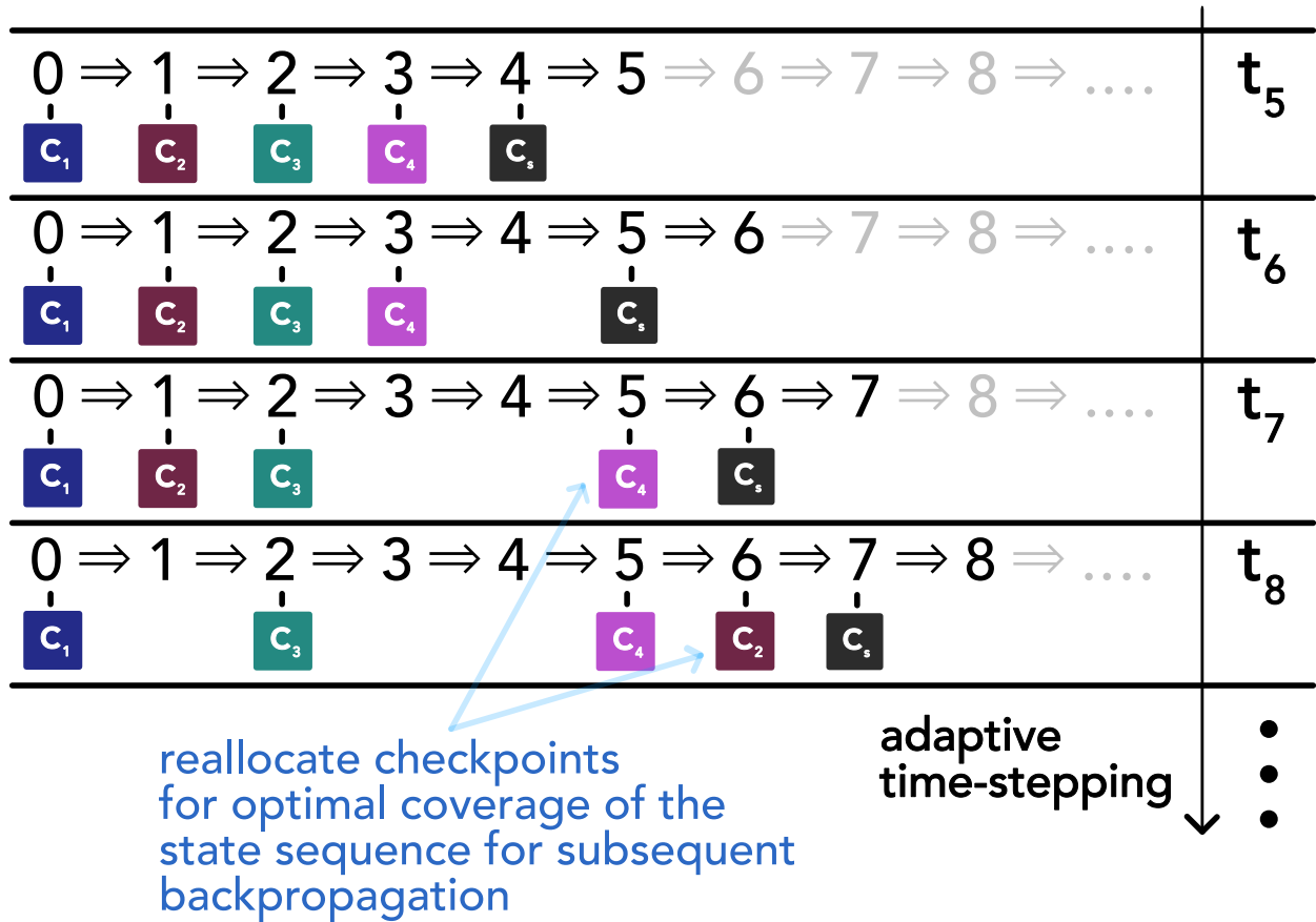
Figure 23: Illustrated is online checkpointing with four checkpoints available, i.e. in a loop with unknown number of iterations how do we reallocate the checkpoints as we go for optimal coverage of the state sequence for subsequent backpropagation. This illustration is based on Fig. 2.2 in Stumm and Walther, 2010. A shadow checkpoint c_s always trails behind the current state. The figure is only meant to give a rough idea, for the details see Algorithm 1 in Stumm and Walther, 2010.
