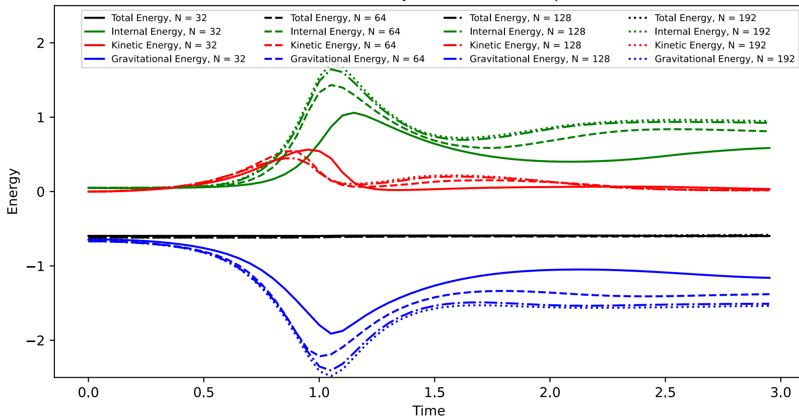
Resolution Study for Evrard's Collapse
