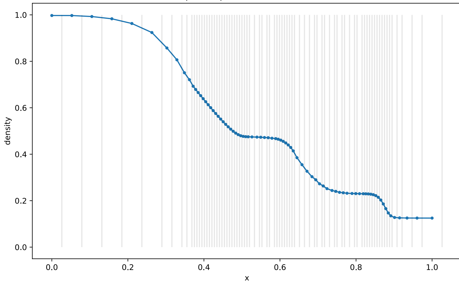
simple adaptive mesh refinement
