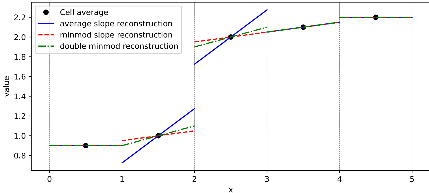
Linear Reconstruction Comparison
