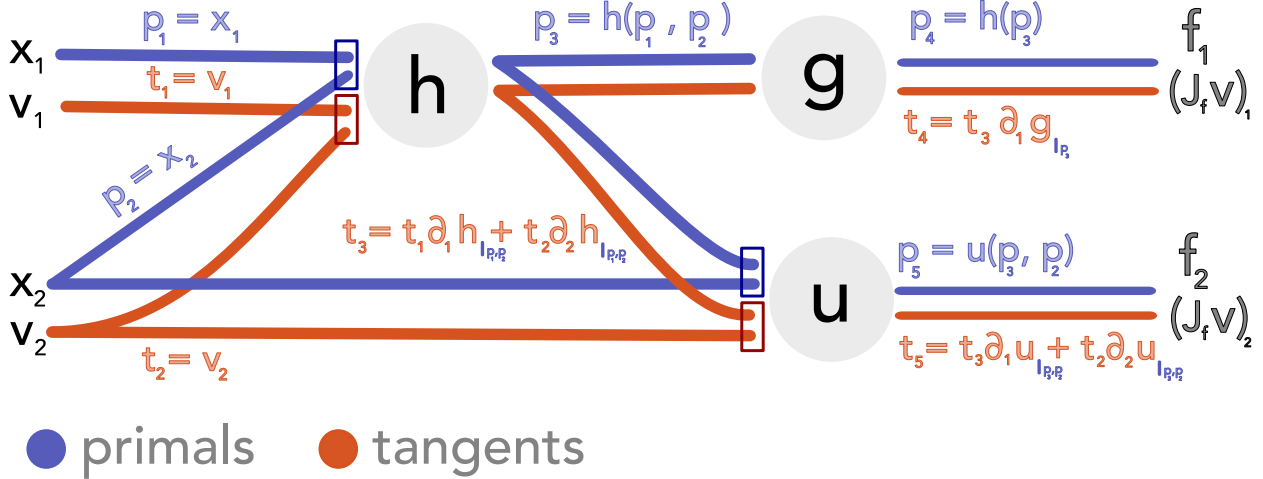
Figure 27: Illustrated is the forward differentiation through the function f (given in Eq. 194). The computational graph is evaluated from left to right, the tangent expressions correspond to the terms of the Jacobian-vector product as given in Eq. 195.
