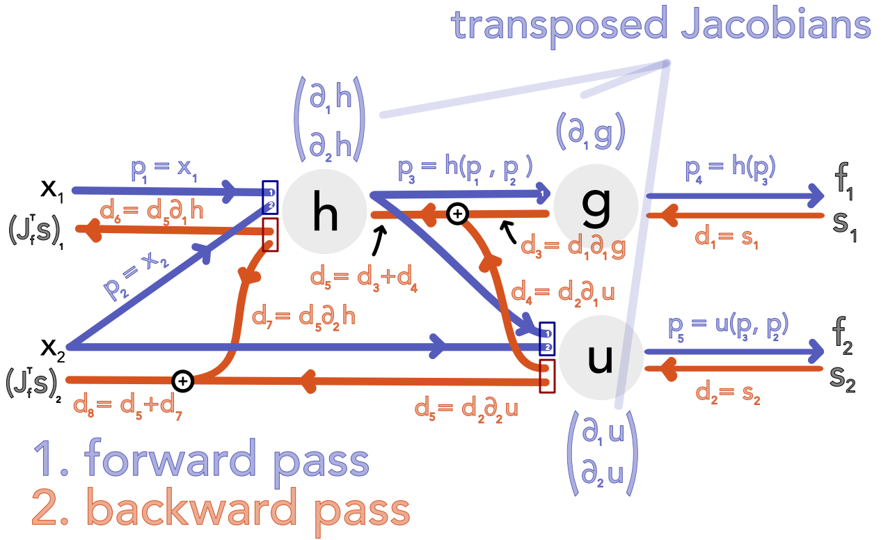
Figure 11: Backward differentiation illustrated for Eq. 98, the result from the backward pass corresponds to the Jacobian transpose vector product in Eq. 101.
