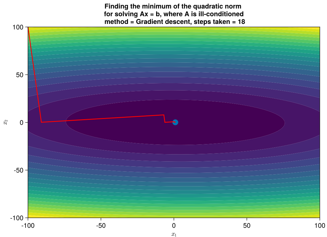
Figure 26: Steepest descent for solving a linear system \underline{\underline{A}}x = \underline{b} with positive definite matrix \underline{\underline{A}} .
