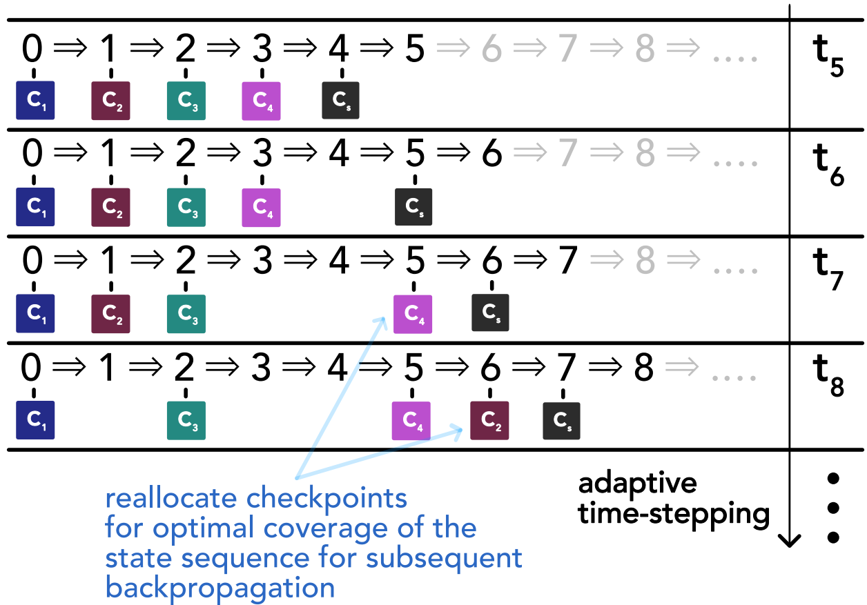
Figure 13: Illustrated is online checkpointing with four checkpoints available, i.e. in a loop with unknown number of iterations how do we reallocate the checkpoints as we go for optimal coverage of the state sequence for subsequent backpropagation. This illustration is based on Fig. 2.2 in Stumm and Walther, 2010. A shadow checkpoint c_s always trails behind the current state. The figure is only meant to give a rough idea, for the details see Algorithm 1 in Stumm and Walther, 2010.
