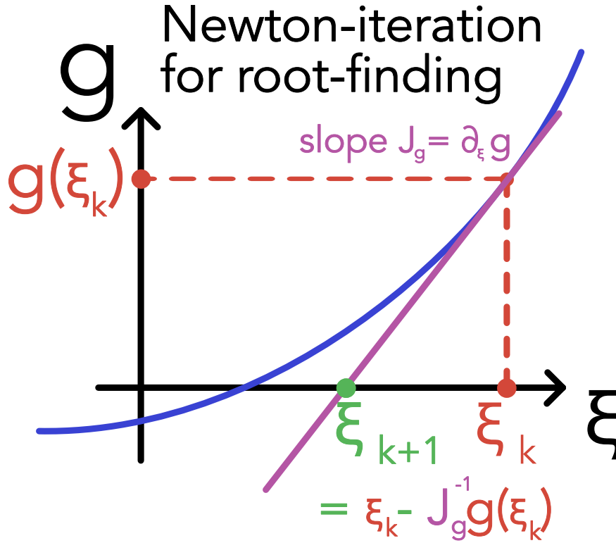
Figure 17: Illustration of the Newton-Raphson method.
