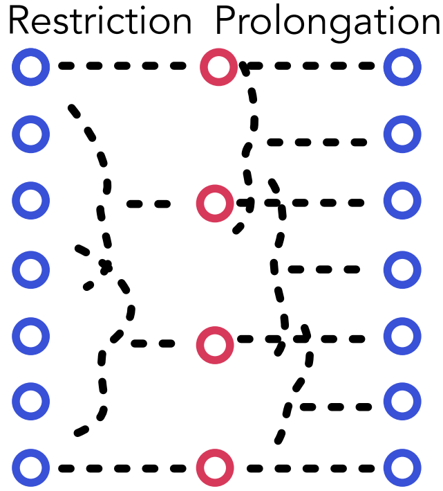
Figure 29: Illustration of restriction and prolongation.
