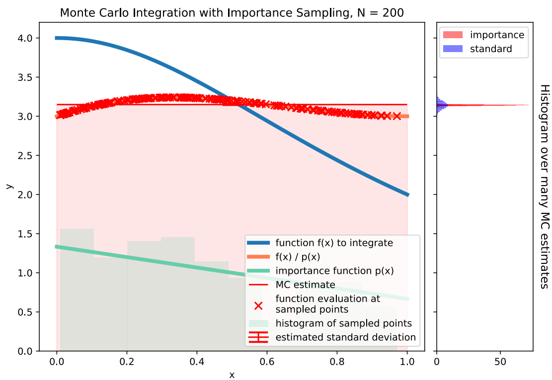
Figure 24: Illustration of Monte Carlo Integration with Importance Sampling for N = 200 samples.
