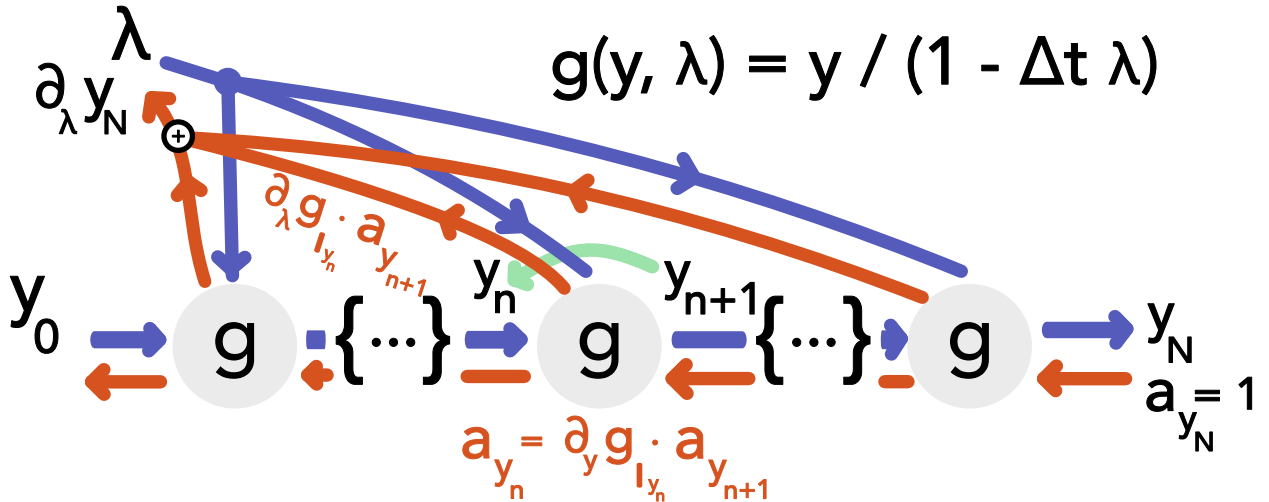
Figure 33: Illustration of backpropagation through the computational graph of an implicit Euler iteration to solve \frac{dy}{dt}(t) = \lambda y(t) , \lambda < 0 , y(0) = y_0 , corresponding to Eq. 268.
