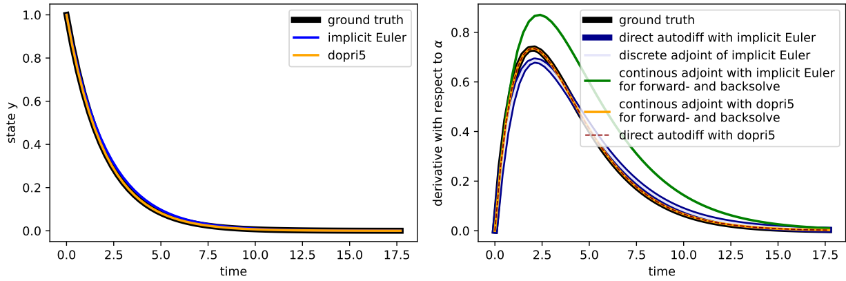
Figure 34: Comparison of different techniques for taking the derivative of the solution to an ODE with respect to its parameters for a simple exponential decay problem.
