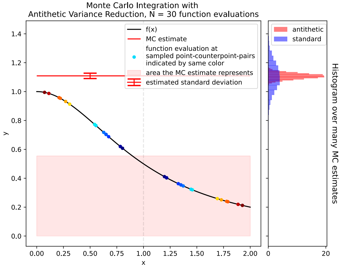
Figure 15: Illustration of Monte Carlo Integration with Antithetic Variables. Notice the even distribution of points around \frac{a+b}{2} = 1 by construction yielding an advantage over the standard Monte Carlo estimator.
