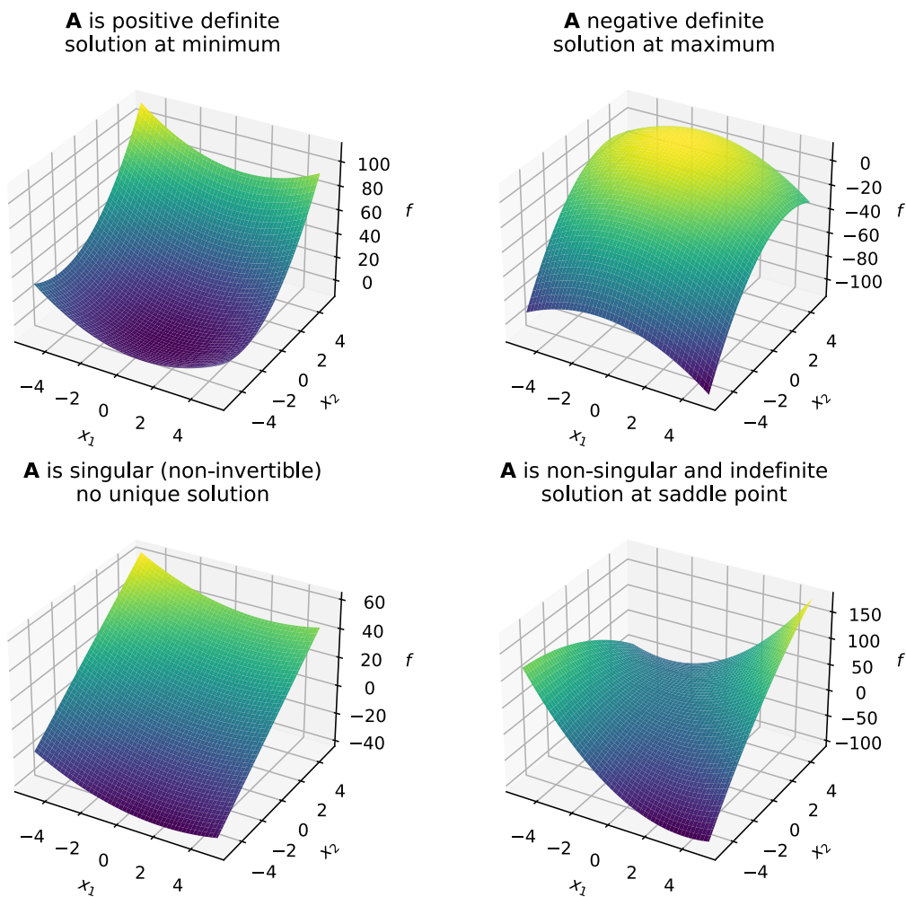
Figure 18: Quadratic forms for different kinds of matrices.
