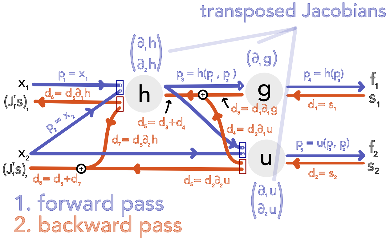
Figure 29: Backward differentiation illustrated for Eq. 245, the result from the backward pass corresponds to the Jacobian transpose vector product in Eq. 248.
