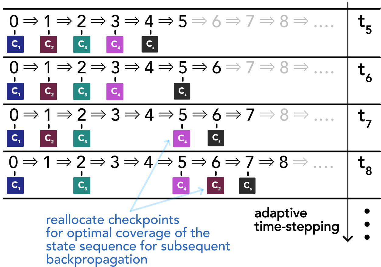
Figure 31: Illustrated is online checkpointing with four checkpoints available, i.e. in a loop with unknown number of iterations how do we reallocate the checkpoints as we go for optimal coverage of the state sequence for subsequent backpropagation. This illustration is based on Fig. 2.2 in Stumm and Walther, 2010. A shadow checkpoint c_s always trails behind the current state. The figure is only meant to give a rough idea, for the details see Algorithm 1 in Stumm and Walther, 2010.
