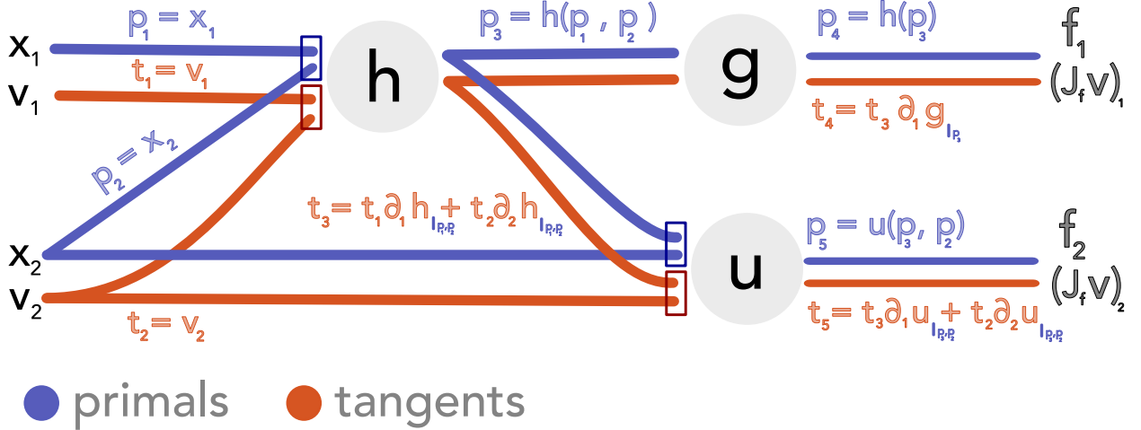
Figure 27: Illustrated is the forward differentiation through the function f (given in Eq. 190). The computational graph is evaluated from left to right, the tangent expressions correspond to the terms of the Jacobian-vector product as given in Eq. 191.
