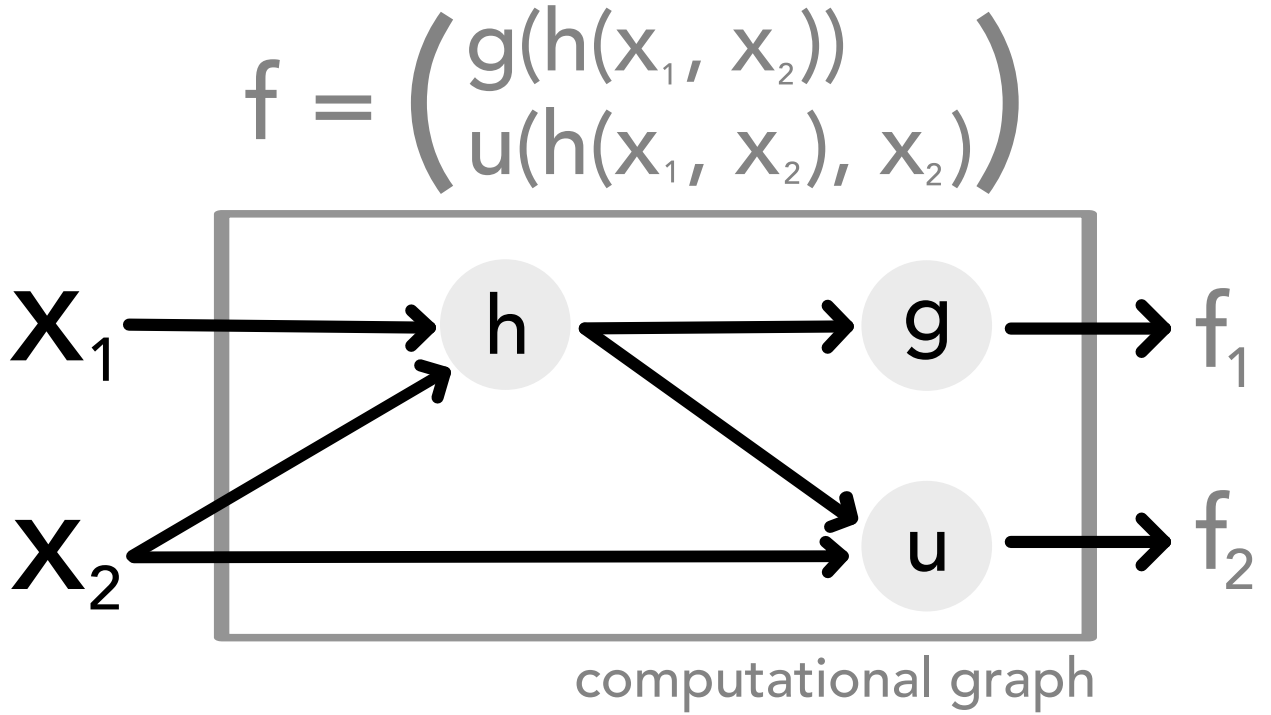
Figure 26: Illustrated is the computational graph of a function f : \mathbb{R}^2 \rightarrow \mathbb{R}^2 (given in Eq. 190) which is composed of functions g : \mathbb{R} \rightarrow \mathbb{R} , h : \mathbb{R}^2 \rightarrow \mathbb{R} , u : \mathbb{R}^2 \rightarrow \mathbb{R} depicted as nodes in the computational graph. Input relations are depicted as arrows.
