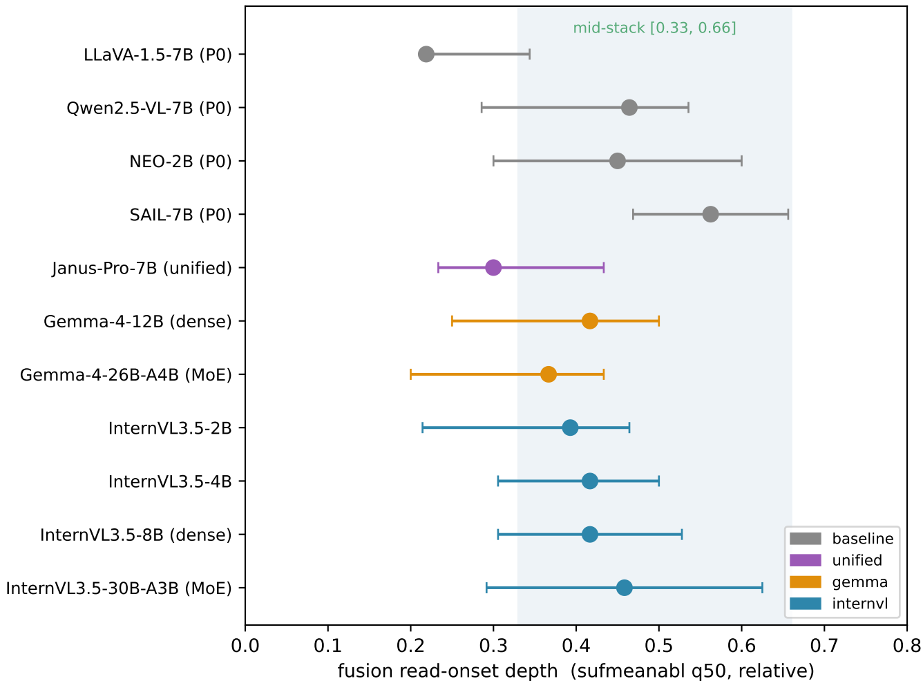
Mid-stack fusion generalizes across MoE / size / unified VLMs
