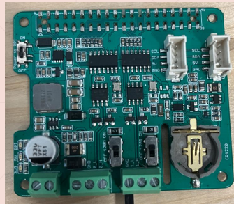
CAN_BUS(FD) Shield(MCP2518FD)
