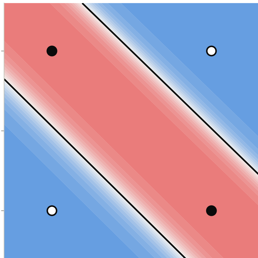
MLP [2, 2, 1] semilla 0: resuelve
