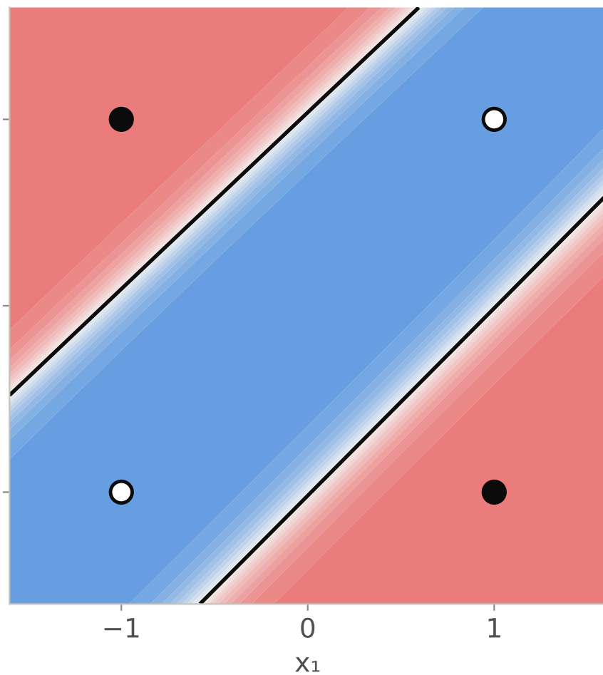
MLP [2, 3, 2, 1] semilla 0: resuelve
