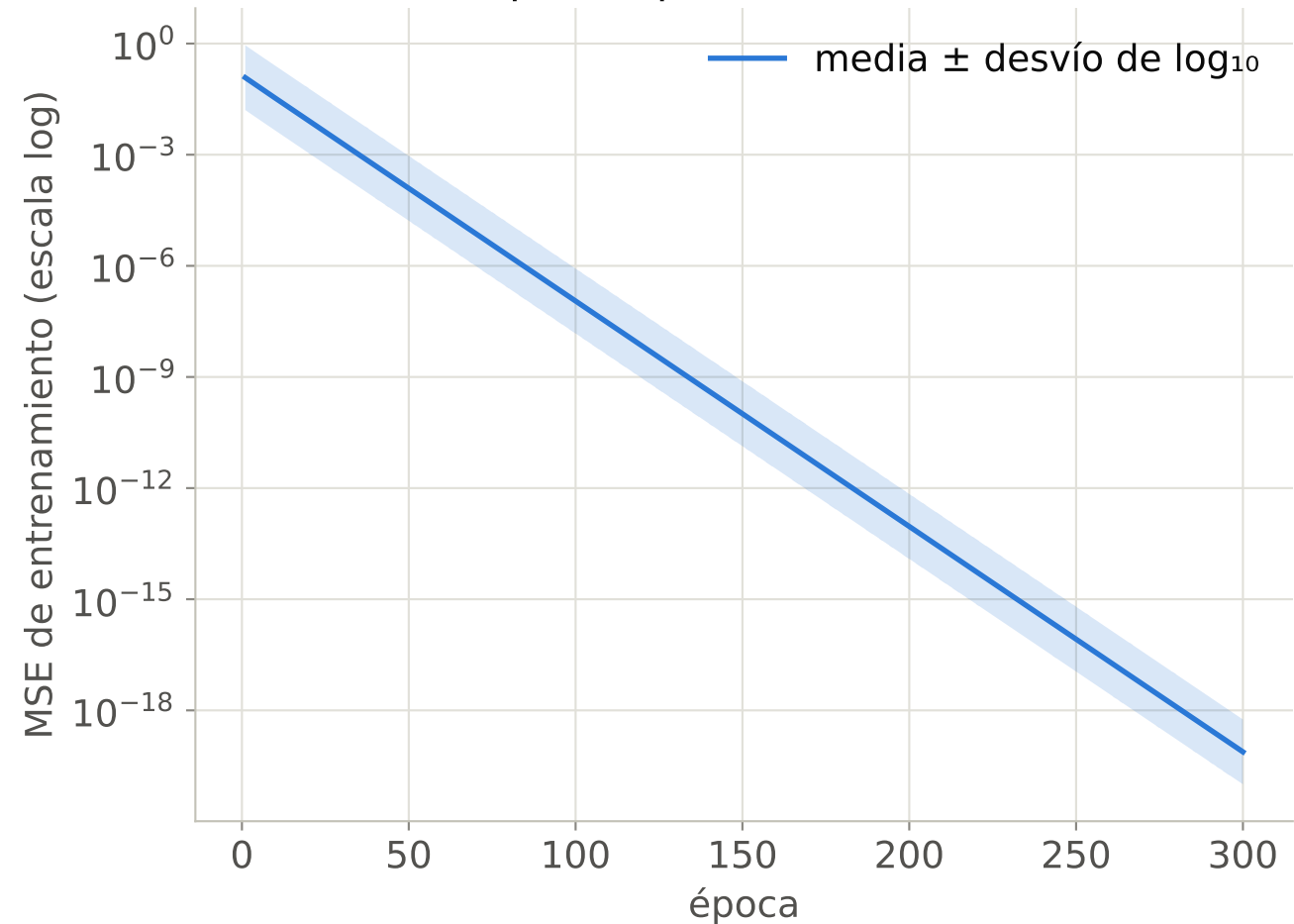
MSE vs época ( \eta = 0.1 , n = 20 semillas)
