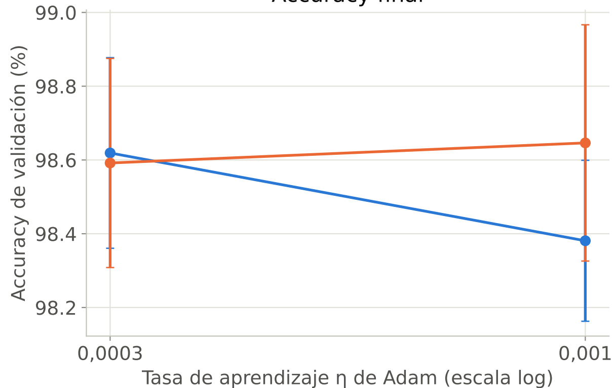
Accuracy final
