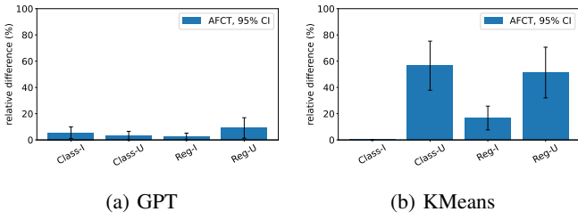
Fig. 6: AFCT relative difference using real traces in Fork.
