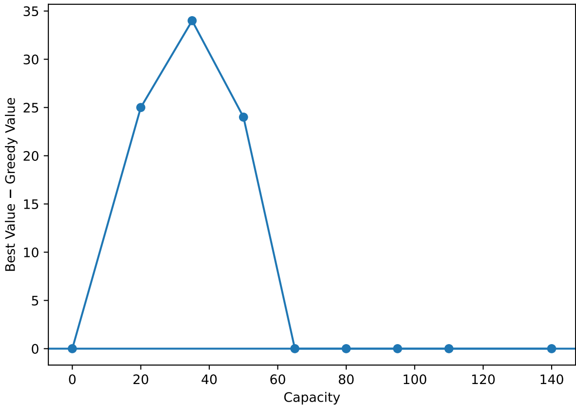
Greedy Value Gap vs Capacity (C1)
