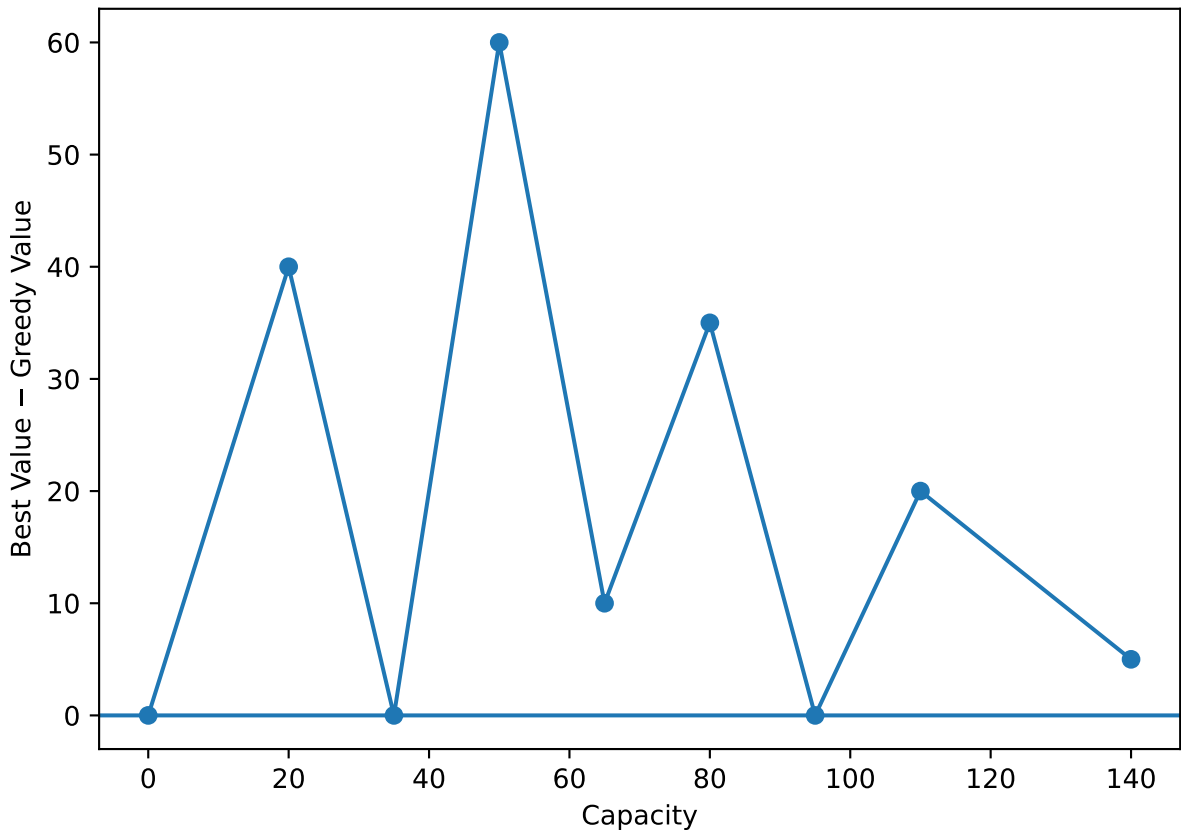
Greedy Value Gap vs Capacity (C2)
