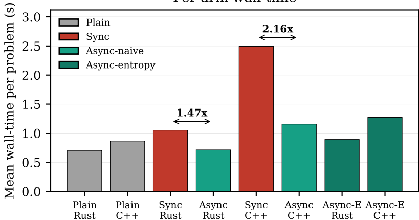
Per-arm wall-time
