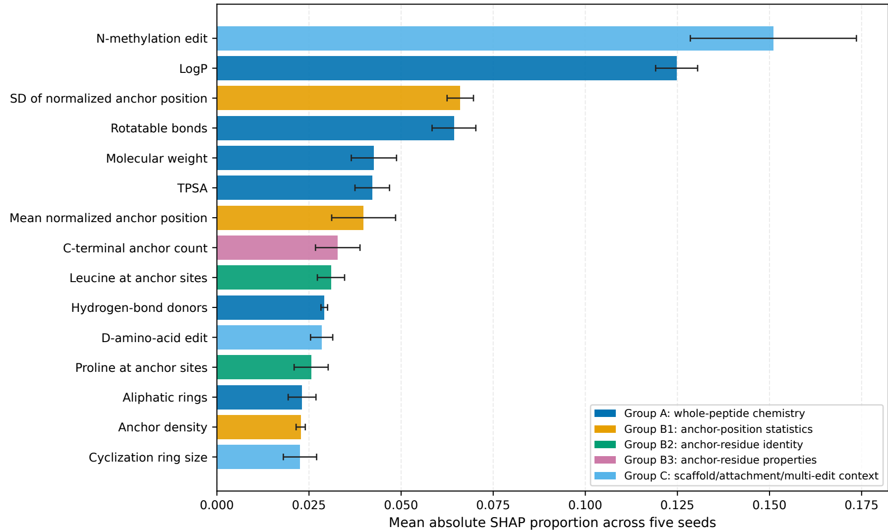
Top individual descriptors in the complete A+B+C representation
