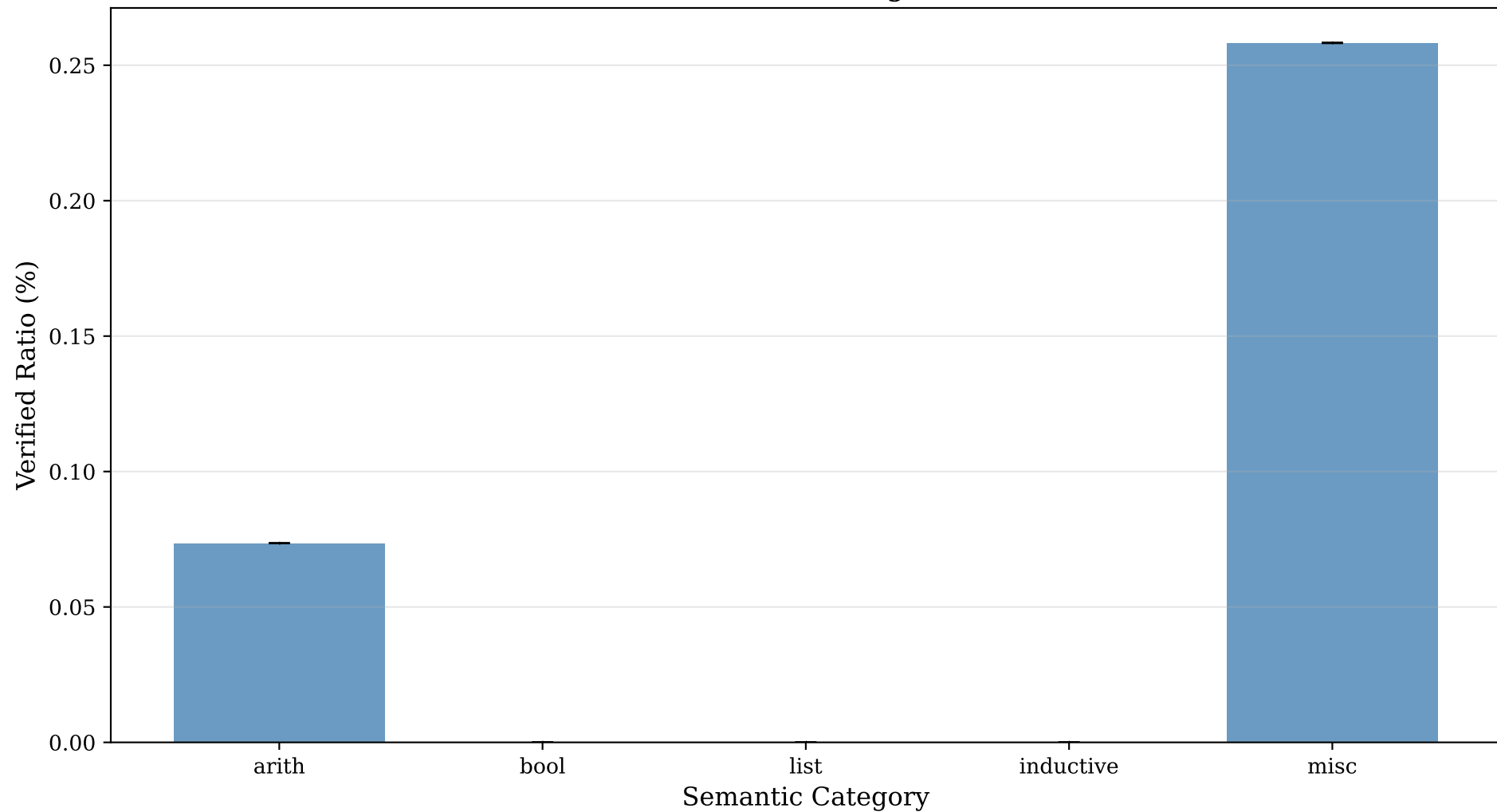
Verified-lemma Ratio by Semantic Category (Verified-Core Configuration)
