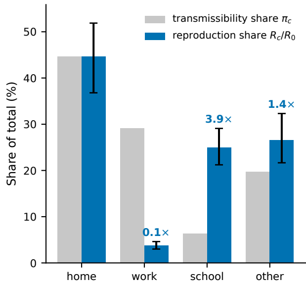
(A) Channel contribution to R_0 vs share
