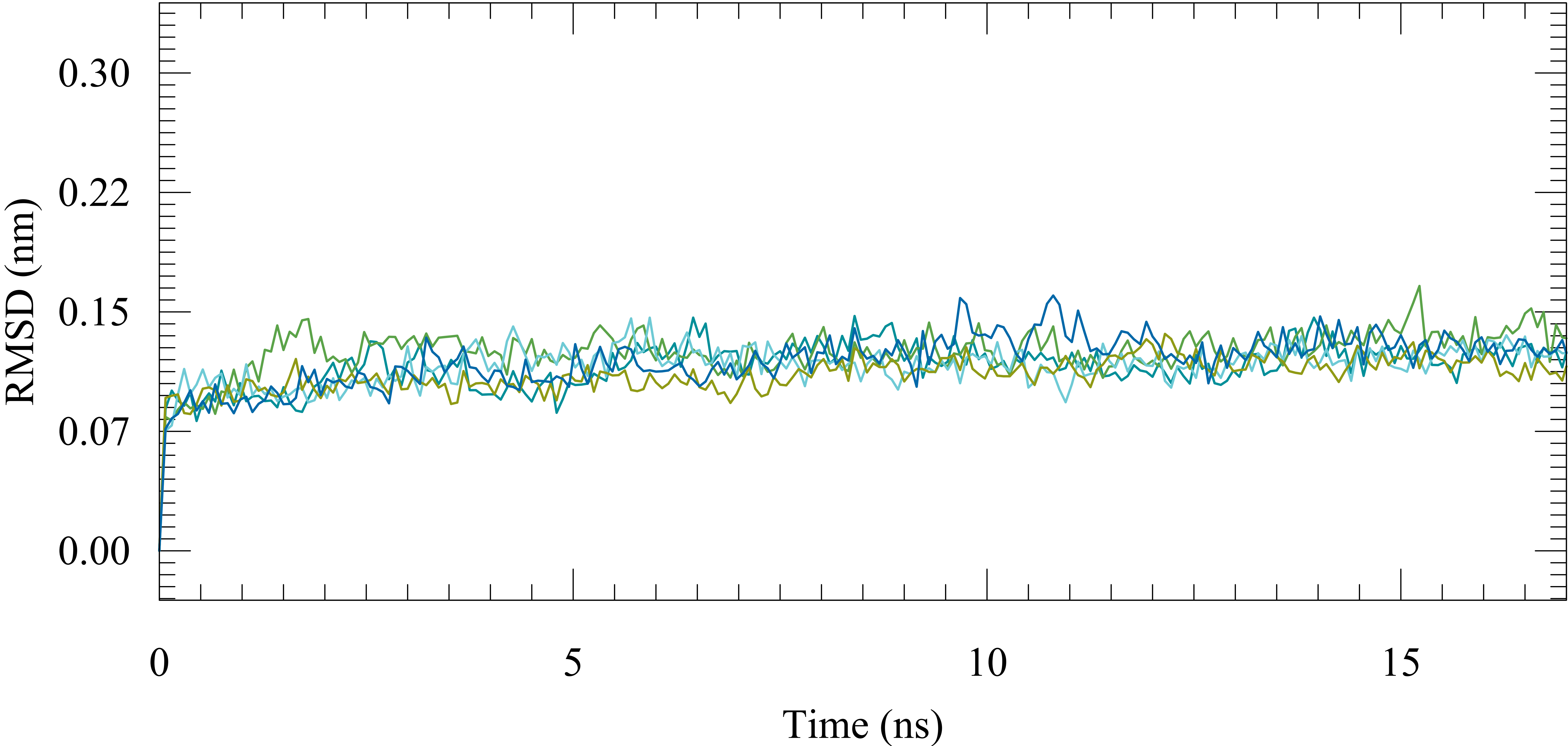
RMSD (Root Mean Square Desviation)
