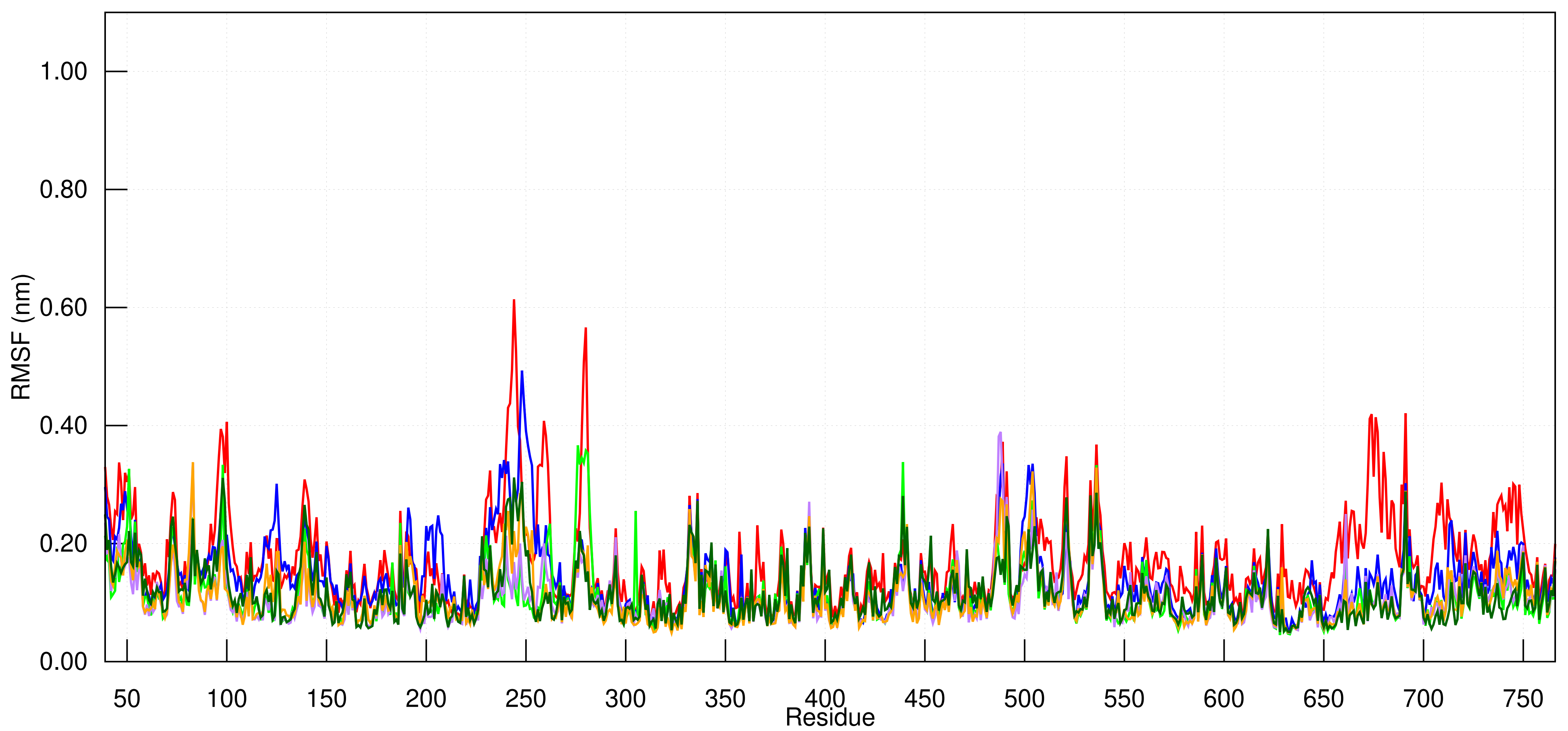
Root Mean Square Fluctuation (RMSF)
