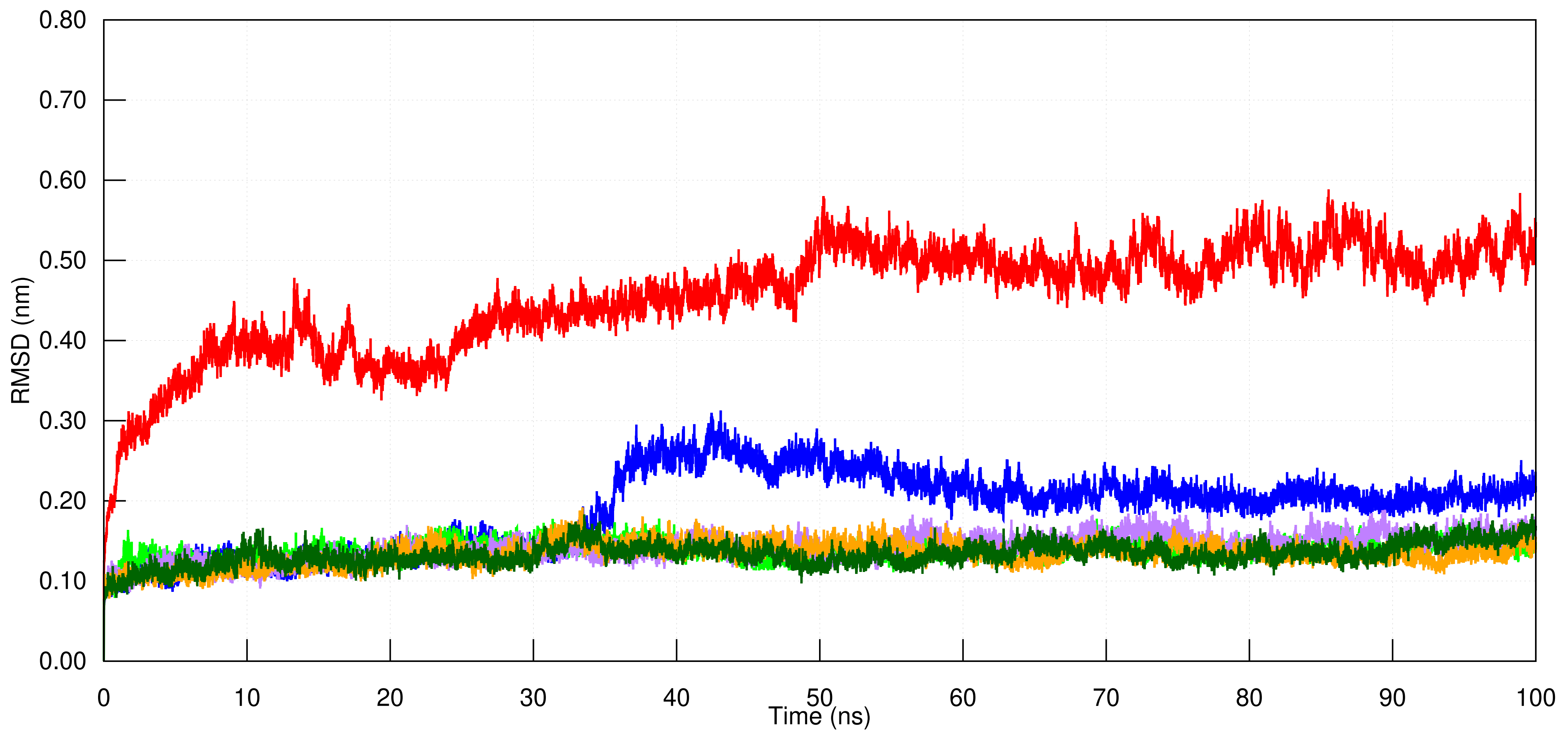
Root Mean Square Deviation (RMSD)
