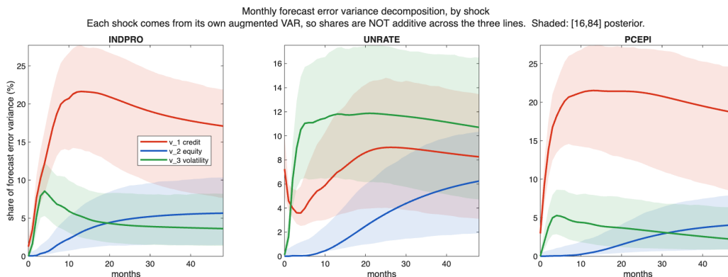
Figure 7: Share of the h -step forecast error variance attributable to each identified shock, with [16,84] posterior bands. Each line comes from its own augmented VAR, so the three are not additive and do not sum to one. The rise of the credit share in industrial production between impact and one year is the transmission chain discussed below.
