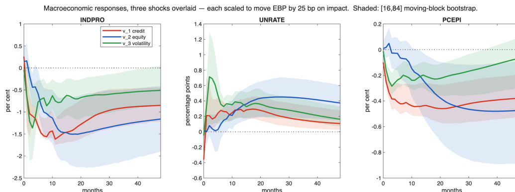
Figure 5: The three shocks on common axes , one panel per macro variable. Each is scaled to move the excess bond premium by 25 basis points on impact, so the vertical distance between the lines is a difference in effect at a common size; shaded areas are [16, 84] moving-block bootstrap bands.
