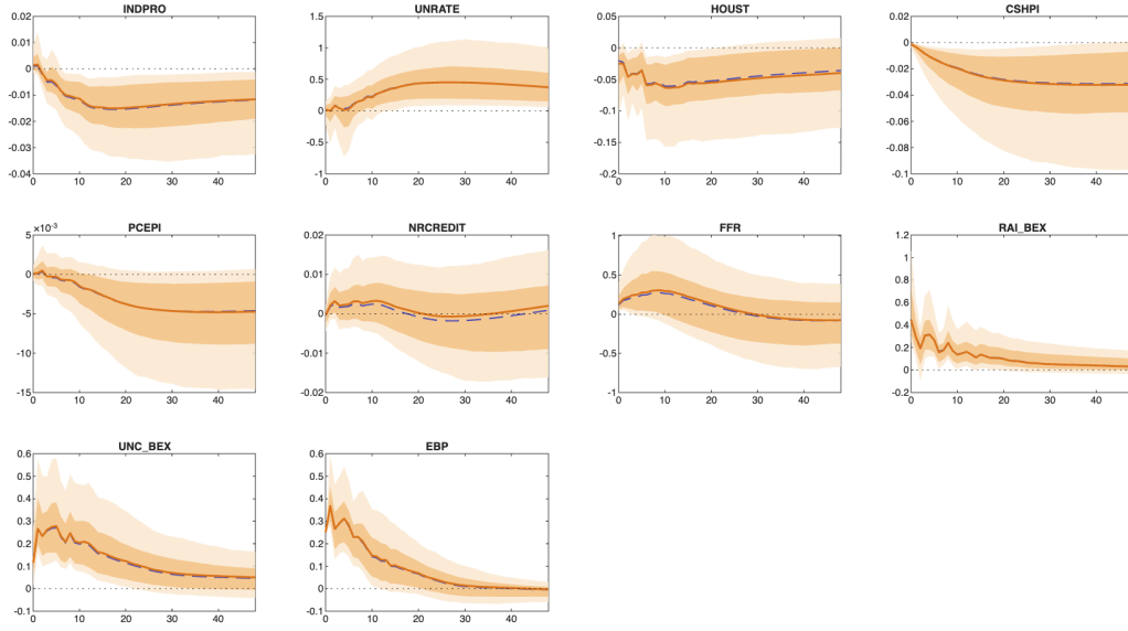
Figure F.3: Macroeconomic impulse responses to the equity shock v_2 , all ten variables. Solid line: Minnesota posterior mean; shaded: [16, 84] and [5, 95] moving-block bootstrap percentiles on the same estimator; dashed: Gaussian posterior band.
