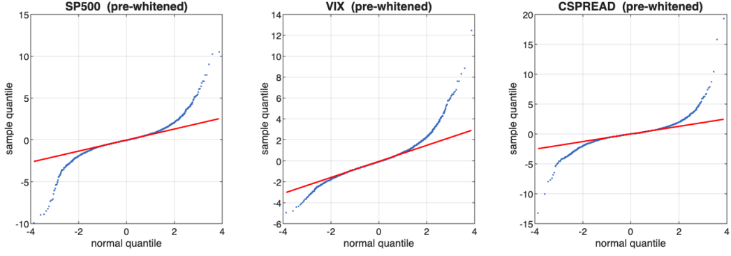
Figure F.5: Normal QQ-plots of the pre-whitened reduced-form residuals \iota_t . The reference line is fitted on the interquartile range rather than by least squares, so that it is not dragged by the tails the plot exists to display.
