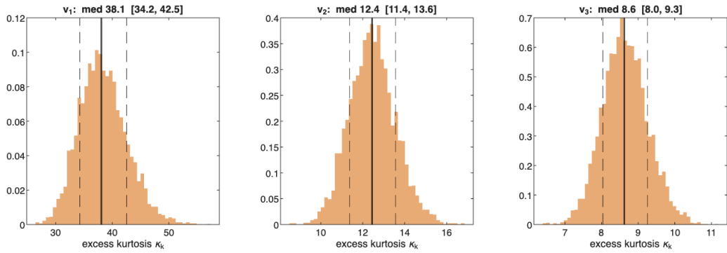
Figure F.7: Posterior distribution of the realised excess kurtosis of each identified shock, over 5,000 draws.
