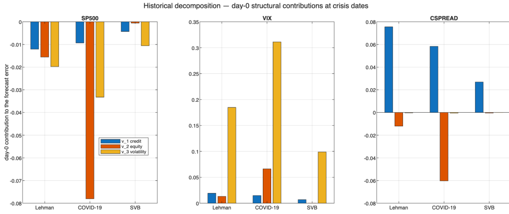
Figure F.1: Structural contributions at the three crisis dates, one bar per shock and variable.
