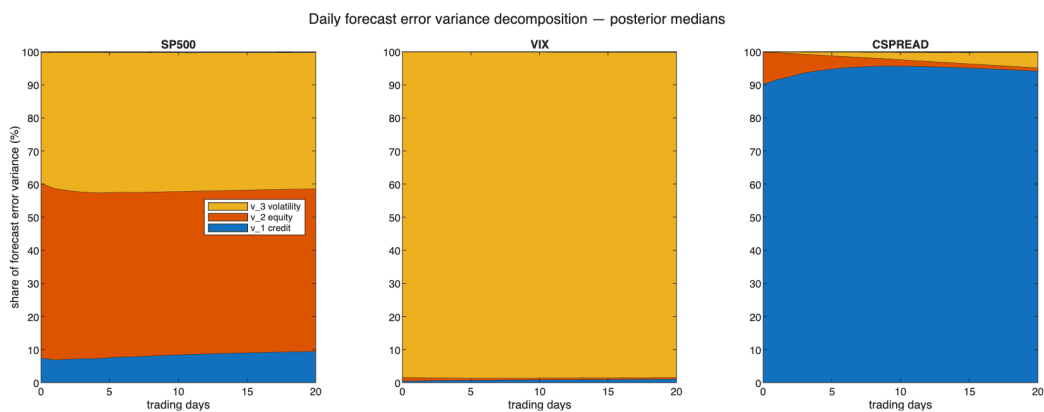
Figure F.8: Daily forecast error variance decomposition , horizon by horizon. Each panel is one system variable; the shaded areas are the shares of its h -step forecast error variance attributable to the three shocks, summing to one at every horizon.
