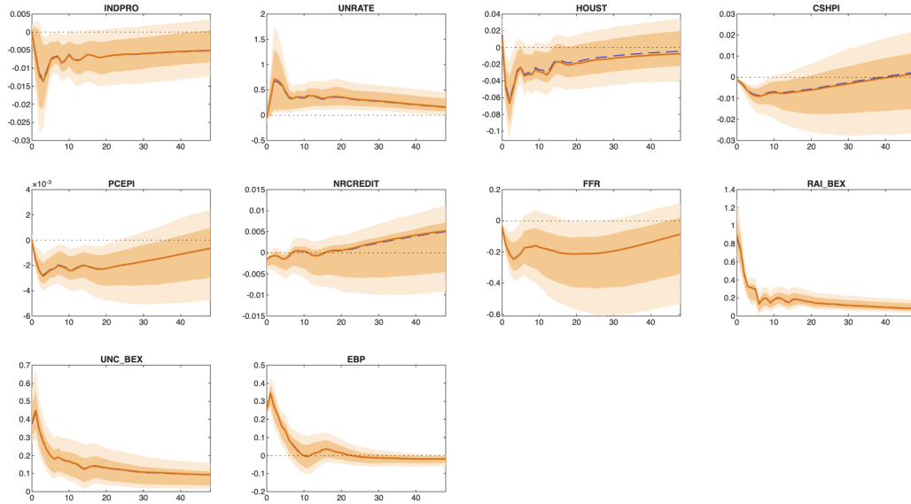
Figure F.4: Macroeconomic impulse responses to the volatility shock v_3 , all ten variables. Conventions as in Figure F.3.
