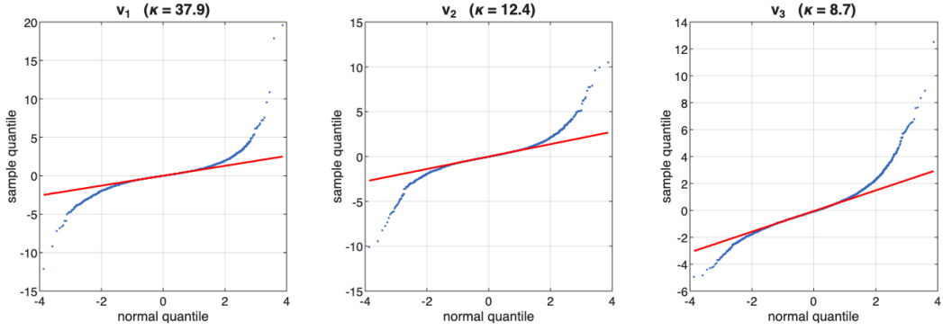
Figure F.6: Normal QQ-plots of the identified structural shocks v_t , each panel labelled by the shock's realised excess kurtosis at the reference identification (37.9, 12.4, 8.7). The posterior medians of the same quantities differ from these in the second significant digit.
