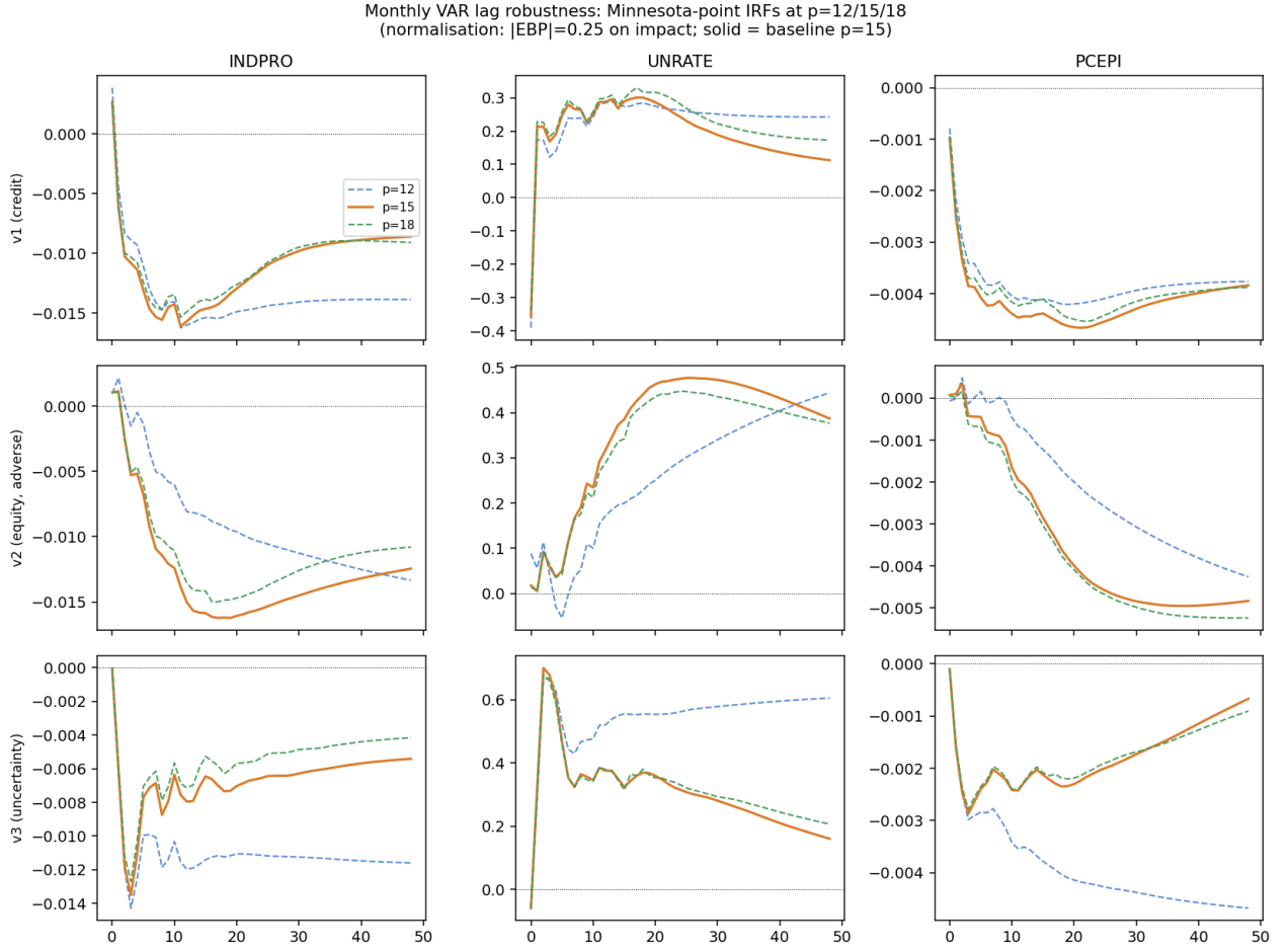
Figure F.2: Impulse responses at p_m = 12, 15 and 18 .
