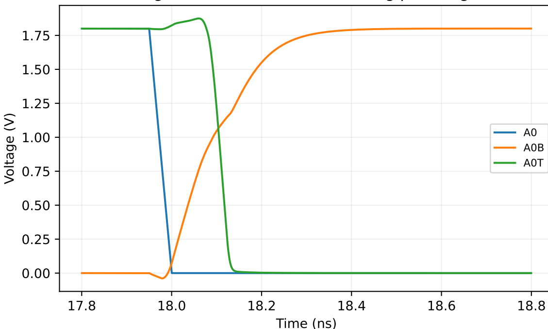
Selected row and unselected WL reference
