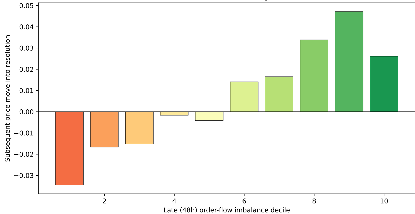
Market-level insider-flow signature
