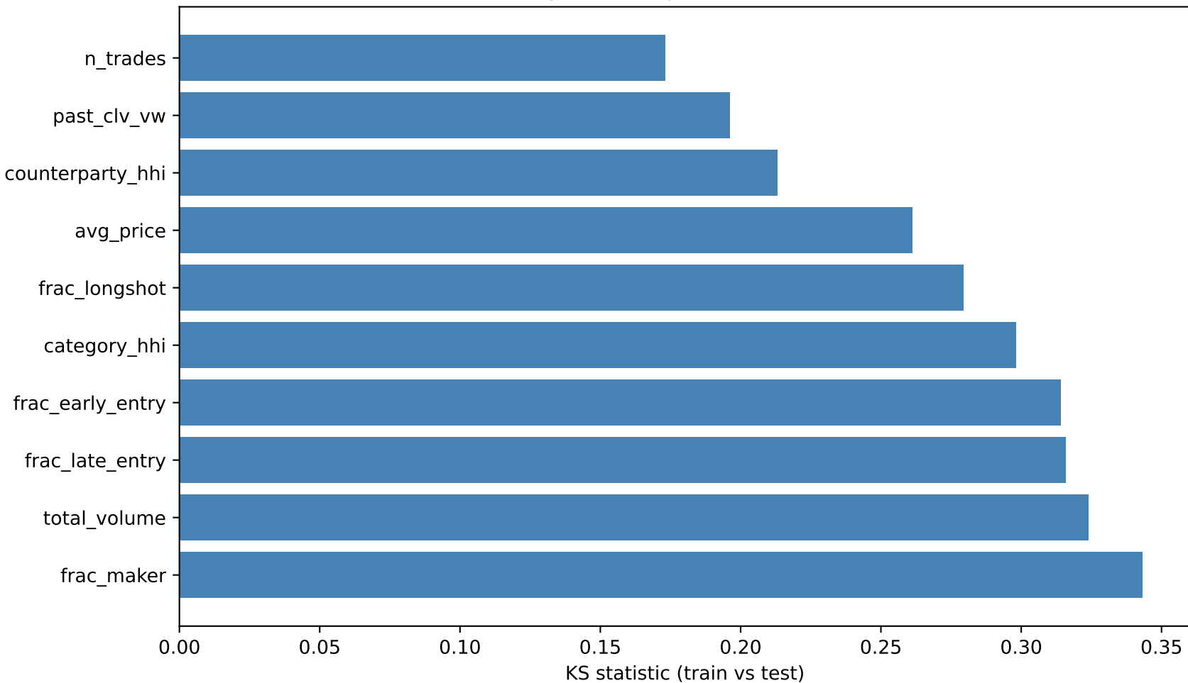
Covariate shift by feature: pooled train vs test (2025-H1)
