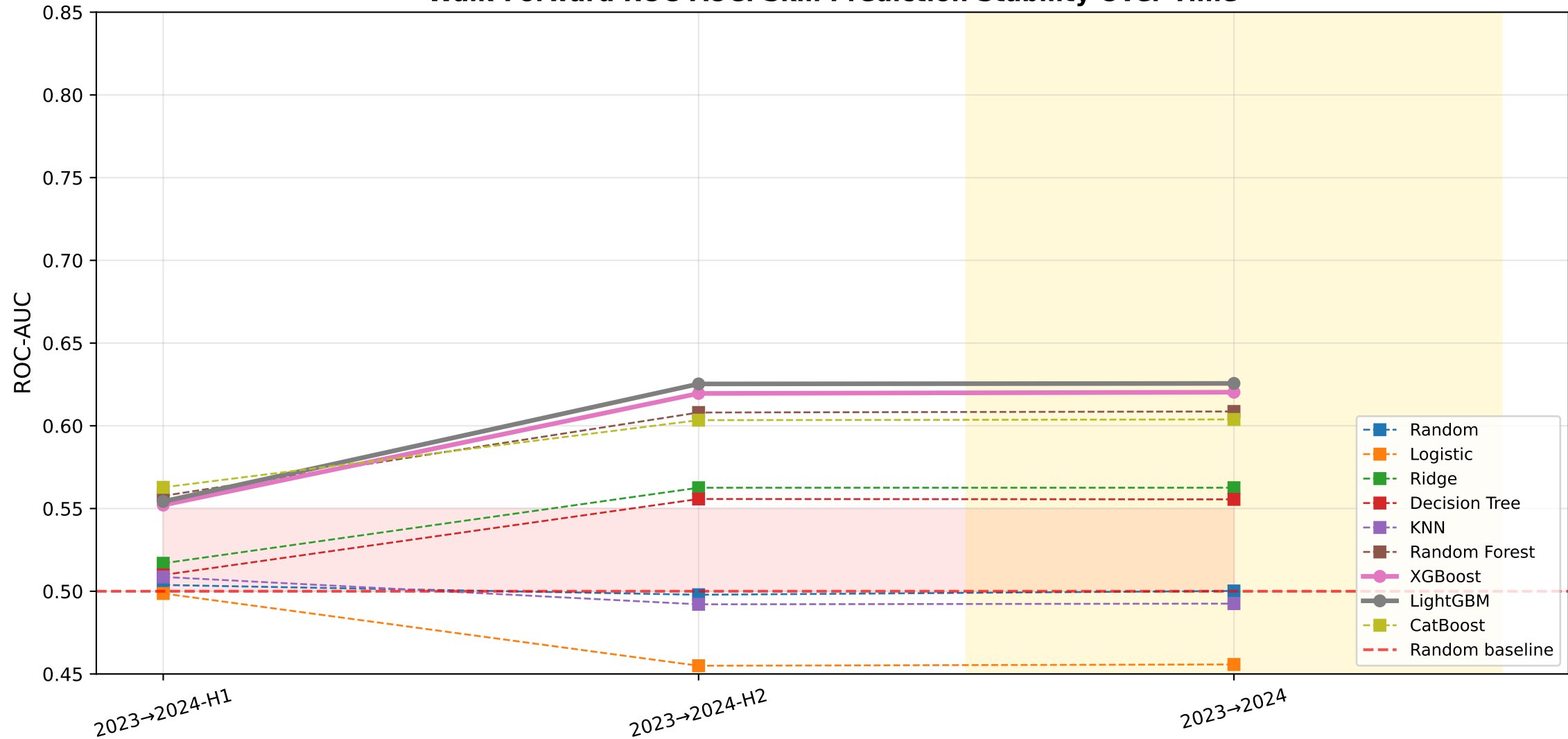
Walk-Forward ROC-AUC: Skill Prediction Stability Over Time
