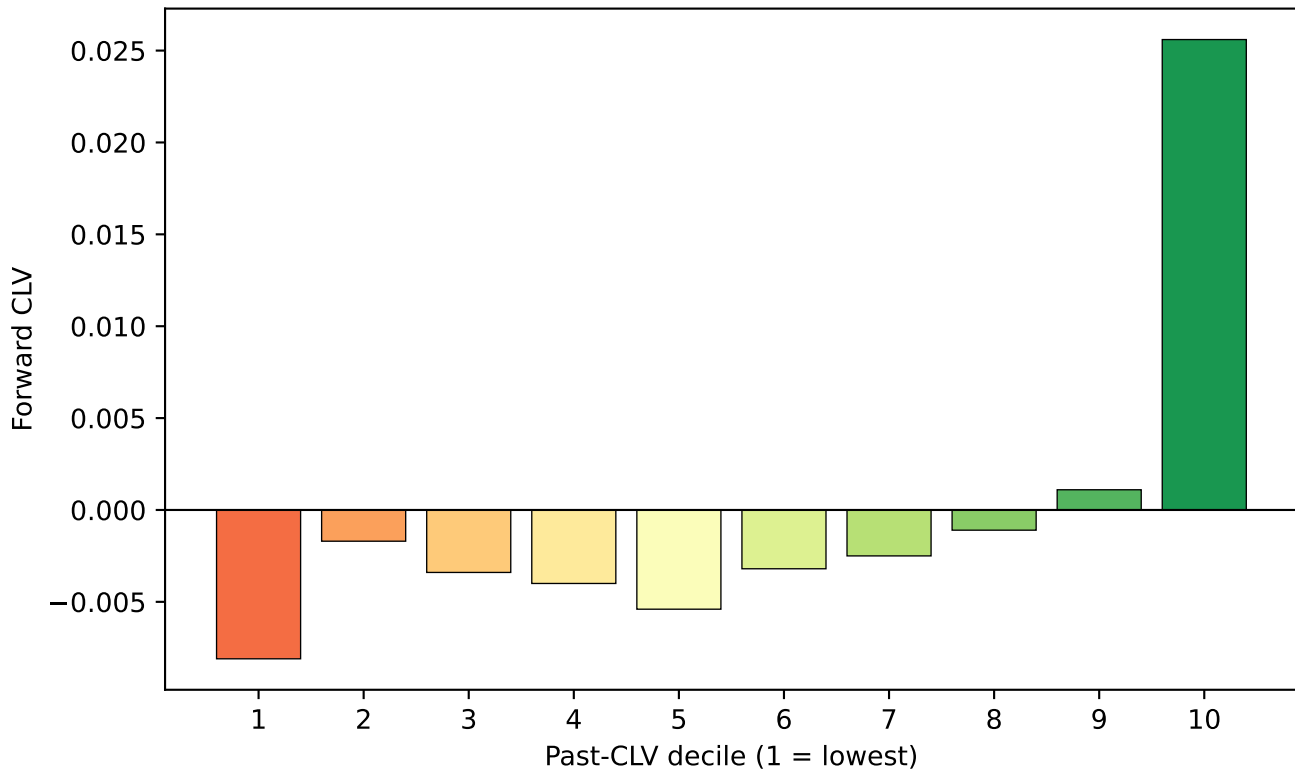
Decile portfolio sort: D10-D1 spread = +0.0337
