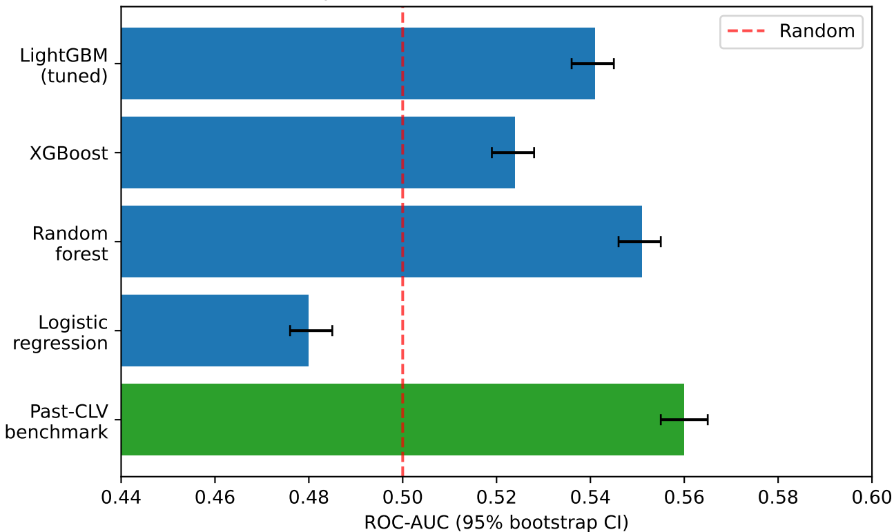
Model comparison, leak-free test window (n=79,329)
