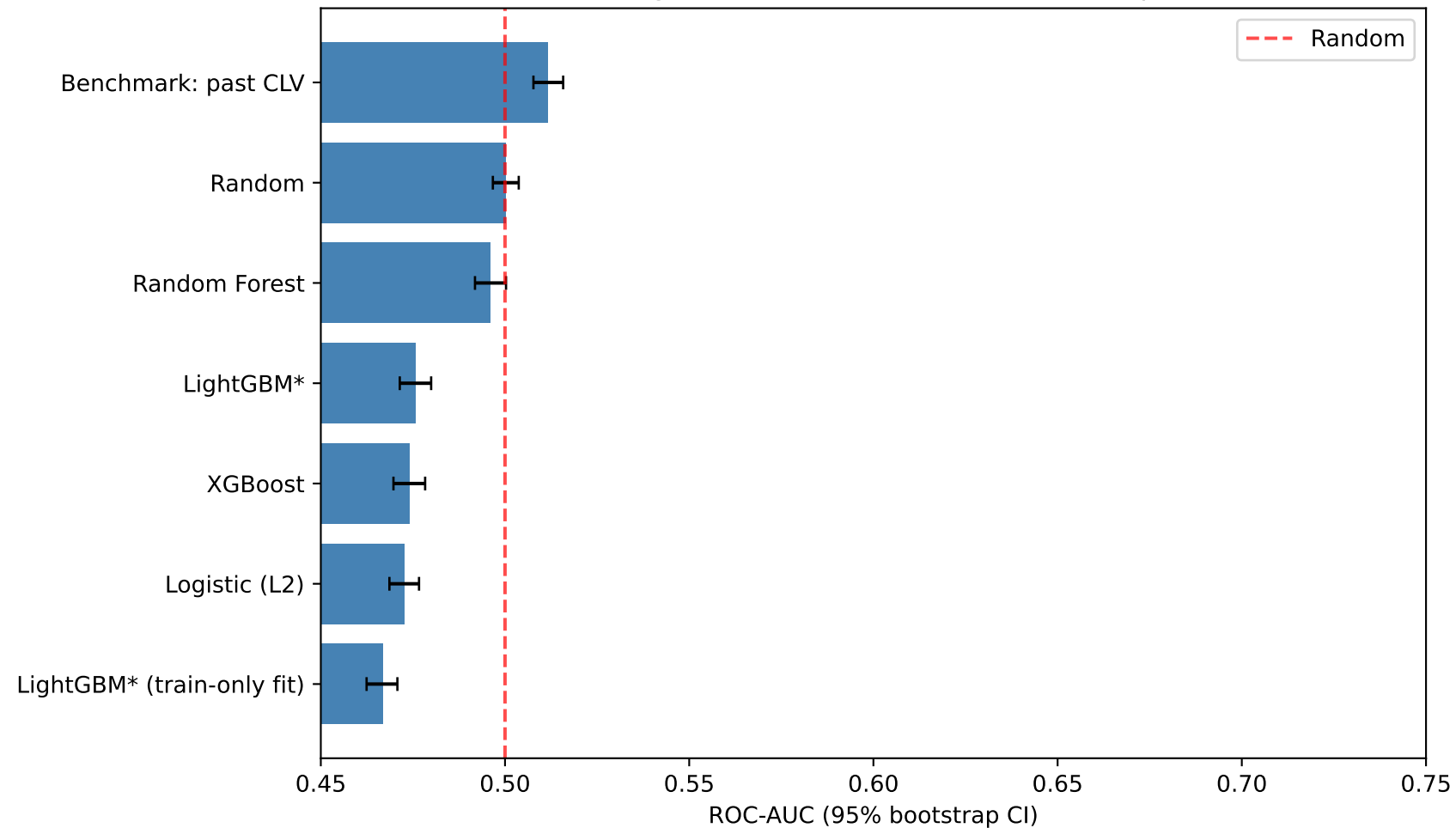
Predicting forward CLV skill — leak-free test panel
